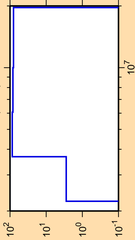
\Delta\sigma/\sigma vs. E for ^{203}\text{Rn}(n,n\alpha)
