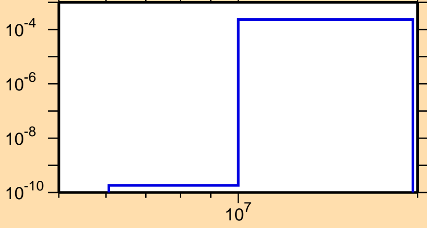
\sigma vs. E for ^{203}\text{Rn}(n,t)
