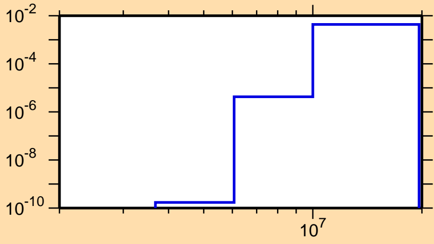
\sigma vs. E for ^{203}\text{Rn}(n,d)
