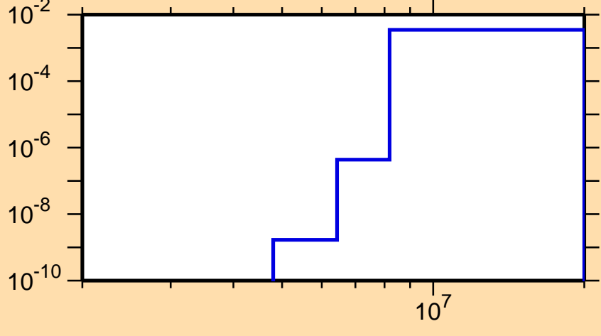
\sigma vs. E for ^{203}\text{Rn}(n,d)
