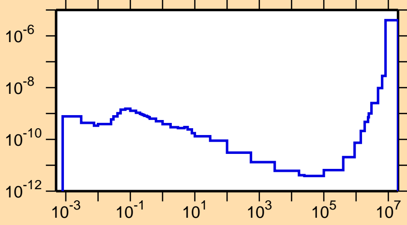
\sigma vs. E for ^{203}\text{Rn}(n,p\alpha)
