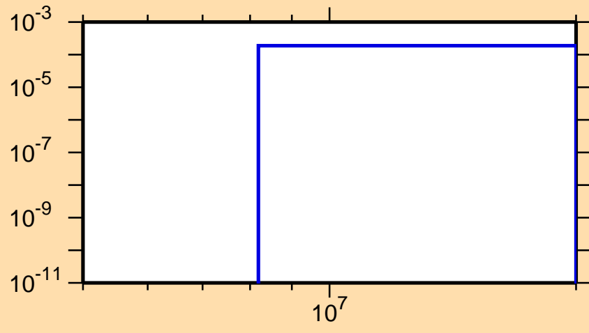
\sigma vs. E for ^{203}\text{Rn}(n,t)
