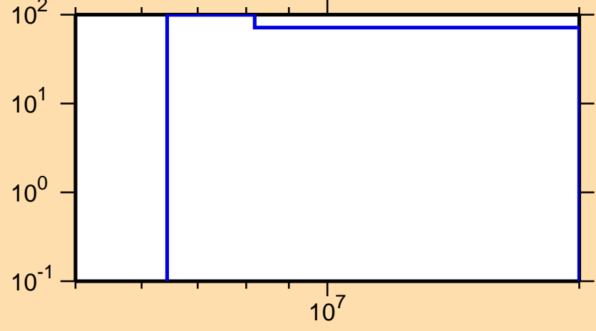
\Delta\sigma/\sigma vs. E for ^{203}\text{Rn}(n,2n)
