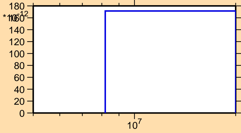
\sigma vs. E for ^{203}\text{Rn}(\text{mt } 45)
