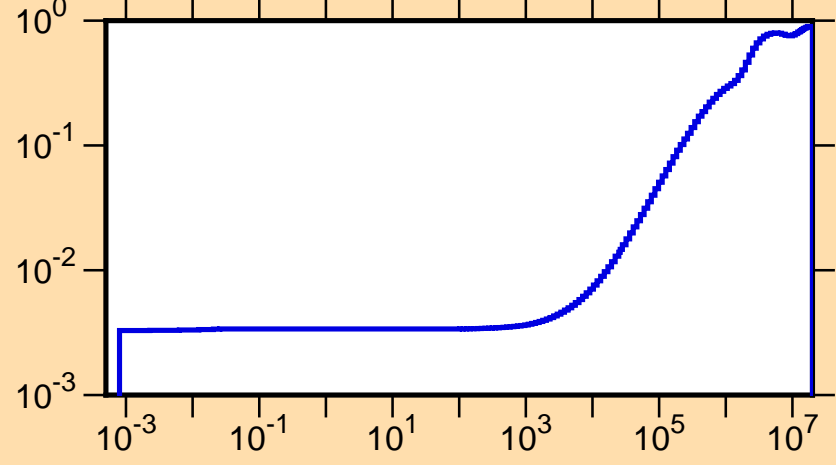
\mu vs. E for ^{205}\text{Rn}(\text{mt251})
