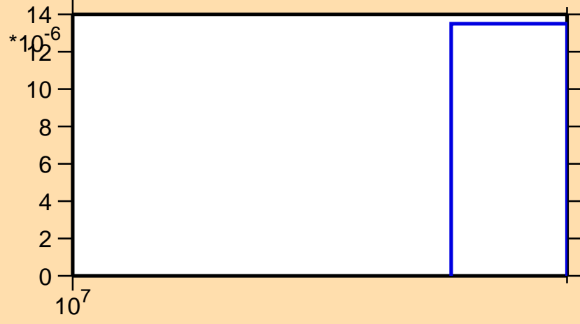
\sigma vs. E for ^{205}\text{Rn}(n,3n)
