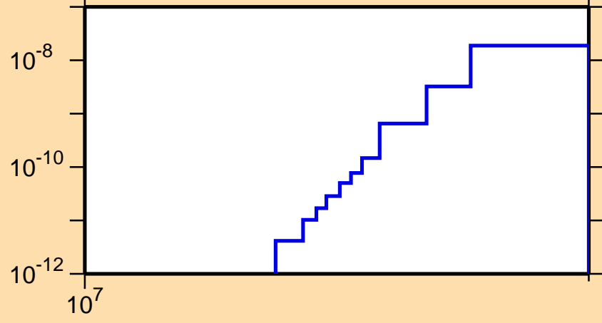
\sigma vs. E for ^{205}\text{Rn}(n,\text{pd})
