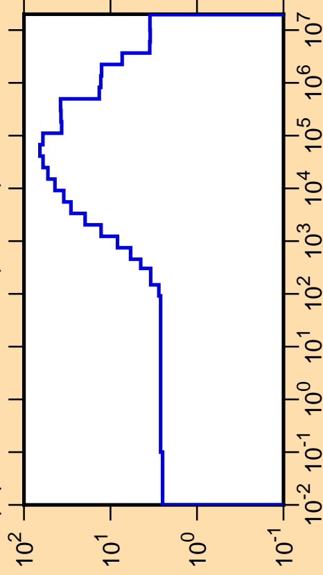
\Delta\mu/\mu vs. E for ^{205}\text{Rn}(\text{mt251})
