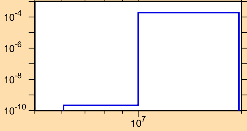
\sigma vs. E for ^{205}\text{Rn}(n,t)
