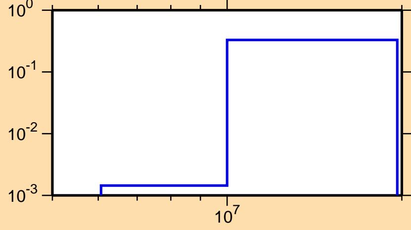
\sigma vs. E for ^{205}\text{Rn}(n,2n)
