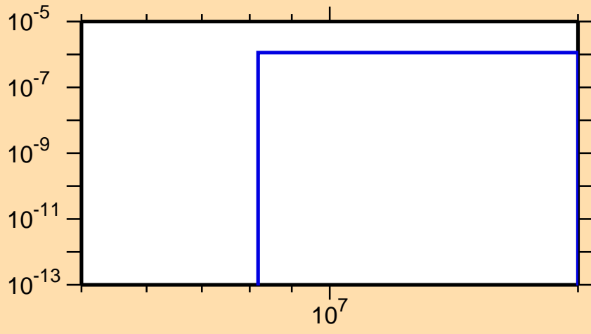
\sigma vs. E for ^{205}\text{Rn} (mt 45)
