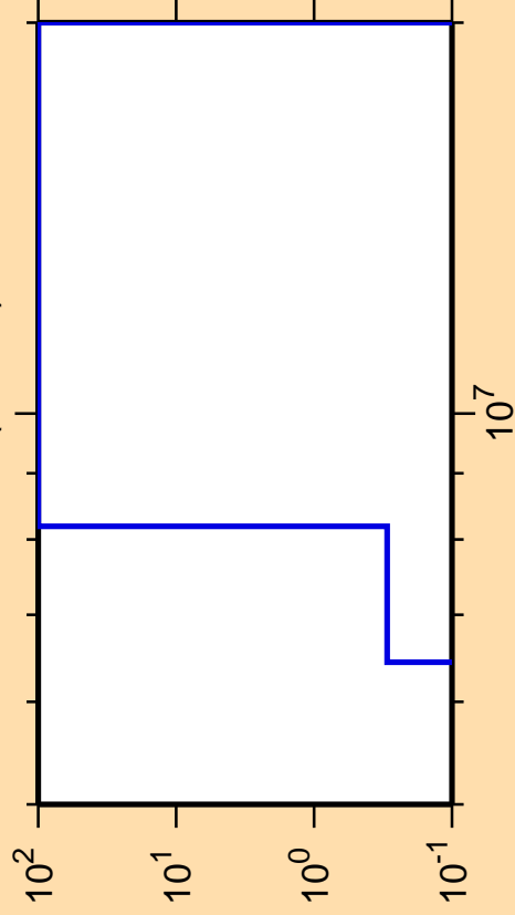
\Delta\sigma/\sigma vs. E for ^{205}\text{Rn} (mt 45)
