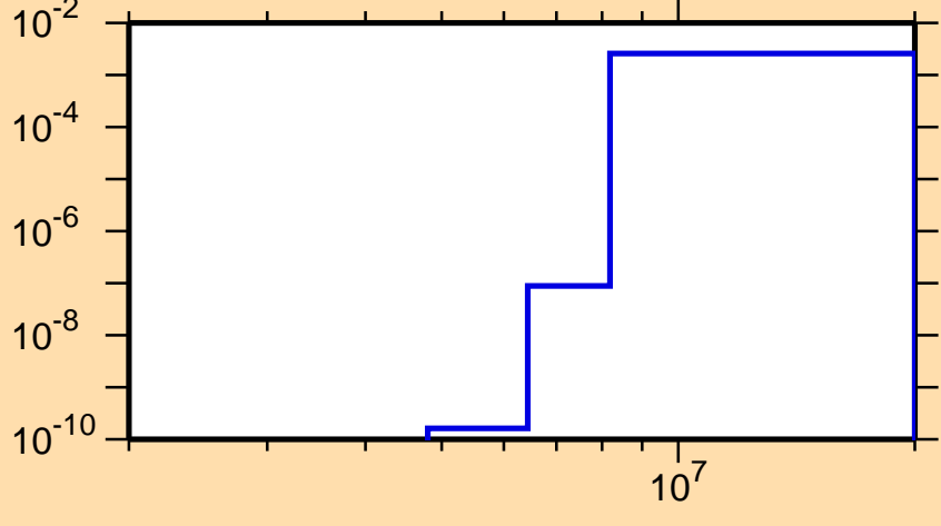
\sigma vs. E for ^{205}\text{Rn}(n,d)
