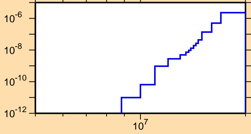
\sigma vs. E for ^{206}\text{Rn}(n,2n\alpha)
