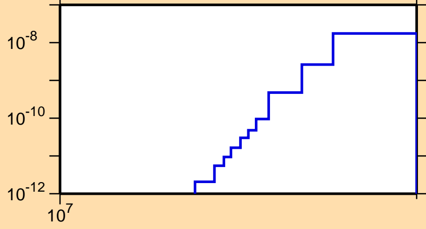
\sigma vs. E for ^{206}\text{Rn}(n,\text{pd})
