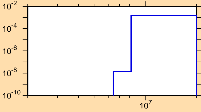
\sigma vs. E for ^{206}\text{Rn}(n,d)
