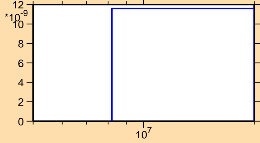
\sigma vs. E for ^{206}\text{Rn}(n,2np)
