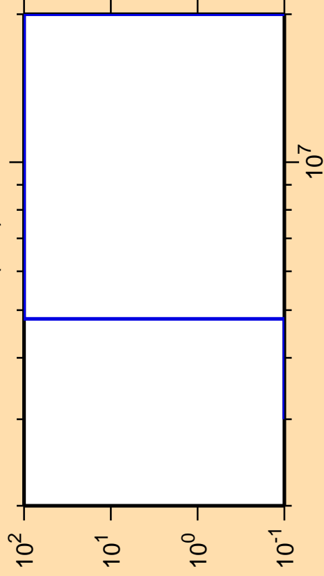
\Delta\sigma/\sigma vs. E for ^{206}\text{Rn}(n,d)
