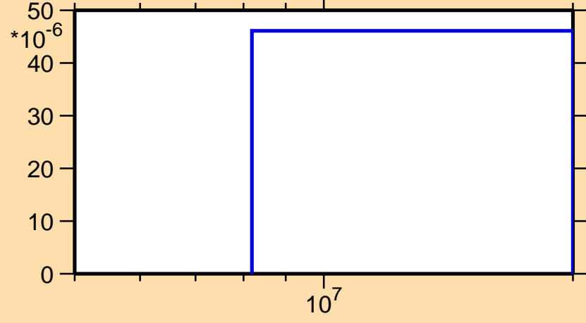
\sigma vs. E for ^{206}\text{Rn}(n,t)
