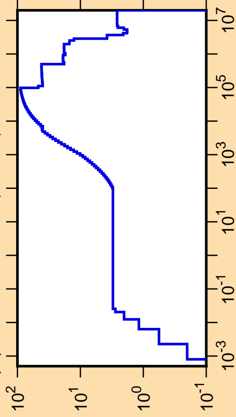
\Delta\mu/\mu vs. E for ^{207}\text{Rn}(\text{mt251})
