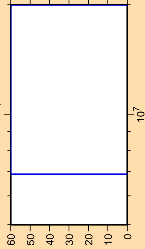
\Delta\sigma/\sigma vs. E for ^{207}\text{Rn}(n,\gamma)
