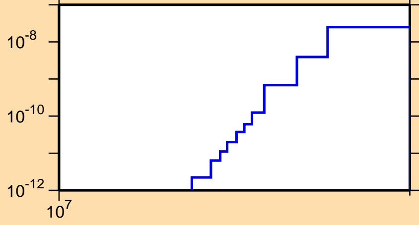
\sigma vs. E for ^{207}\text{Rn}(n,\text{pd})
