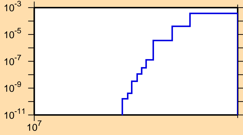
\sigma vs. E for ^{207}\text{Rn}(n,2np)
