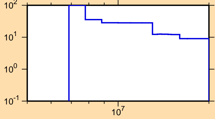
\Delta\sigma/\sigma vs. E for ^{207}\text{Rn}(n,2n)
