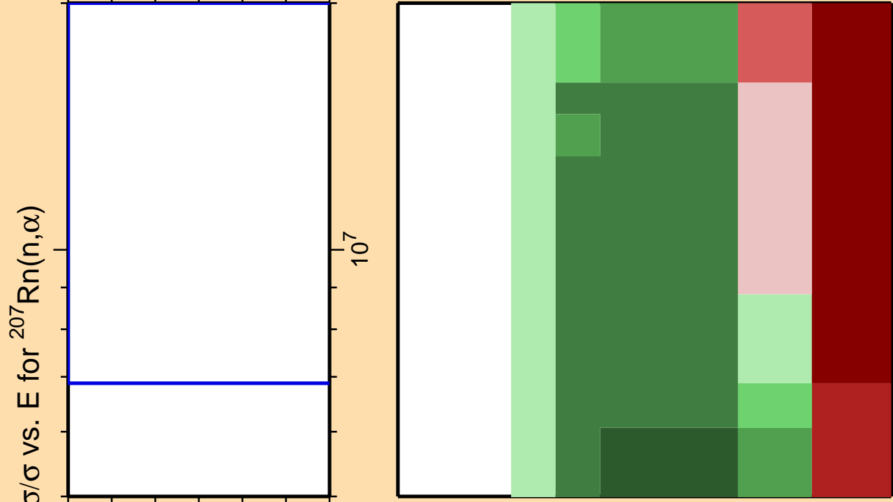
\Delta\sigma/\sigma vs. E for ^{207}\text{Rn}(n,2n)
