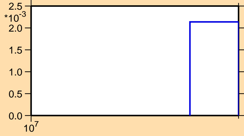
\sigma vs. E for ^{207}\text{Rn}(n,3n)
