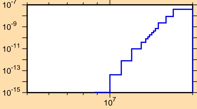
\sigma vs. E for ^{207}\text{Rn}(\text{mt } 45)
