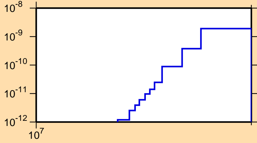
\sigma vs. E for ^{207}\text{Rn}(\text{mt117})
