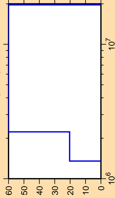
\Delta\sigma/\sigma vs. E for ^{207}\text{Rn}(n,n\alpha)
