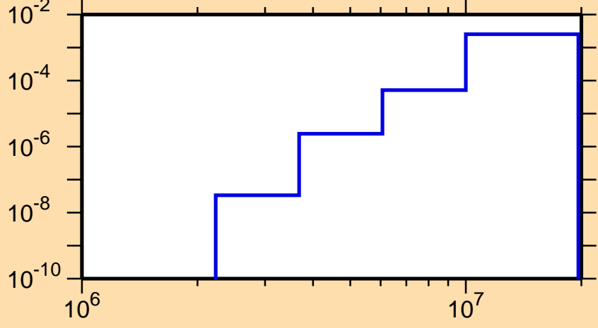
\sigma vs. E for ^{207}\text{Rn}(n,n\alpha)
