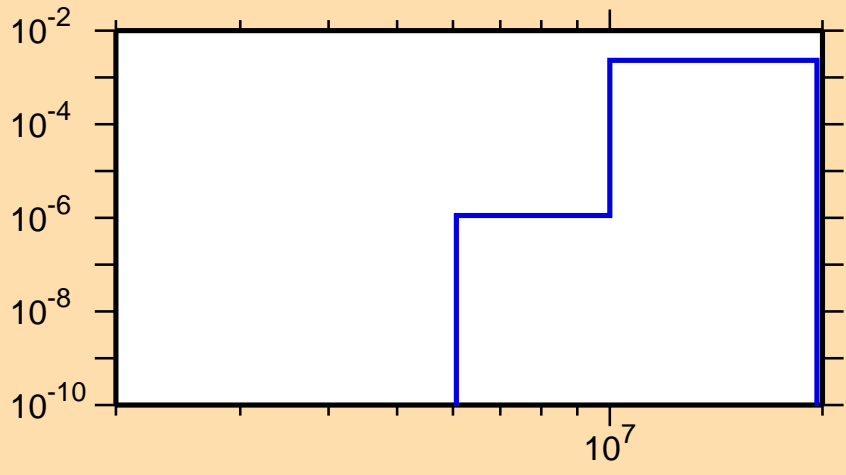
\sigma vs. E for ^{207}\text{Rn}(n,d)
