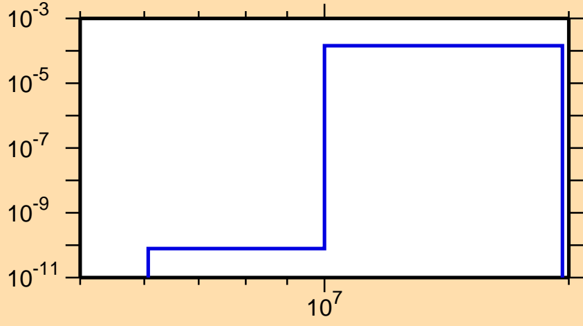
\sigma vs. E for ^{207}\text{Rn}(n,t)
