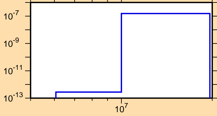
\sigma vs. E for ^{207}\text{Rn}(n,\text{He}3)
