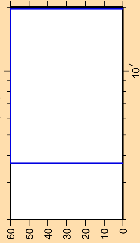
\Delta\sigma/\sigma vs. E for ^{207}\text{Rn}(n,d)
