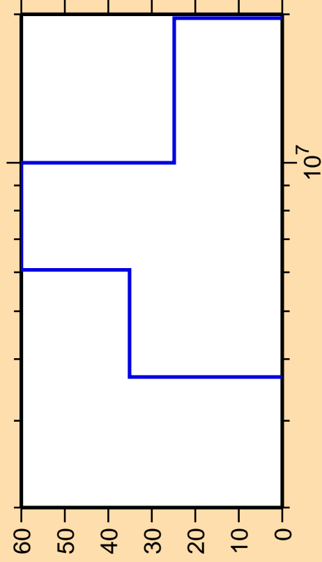
\Delta\sigma/\sigma vs. E for ^{207}\text{Rn}(n,np)
