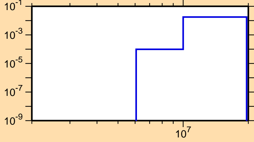
\sigma vs. E for ^{207}\text{Rn}(n,np)
