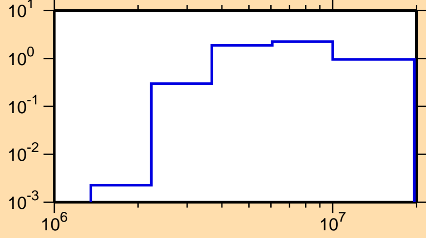
\sigma vs. E for ^{207}\text{Rn}(n,n\text{cont.})
