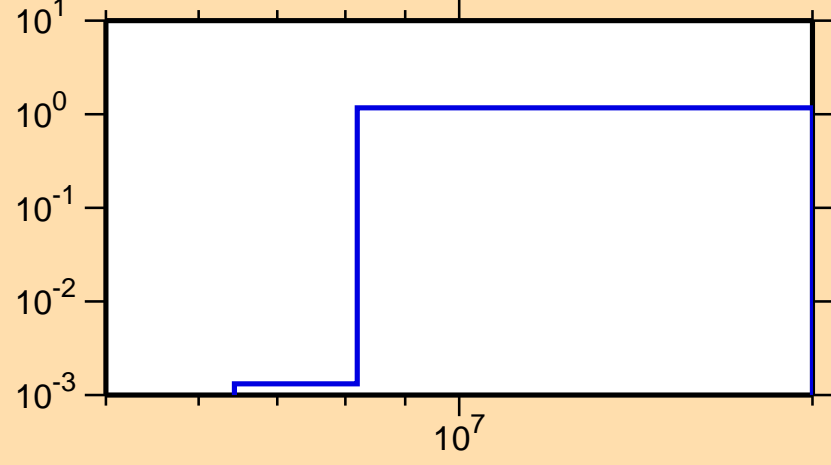
\sigma vs. E for ^{207}\text{Rn}(n,2n)
