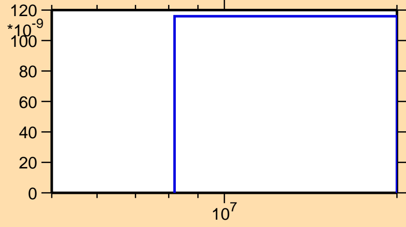
\sigma vs. E for ^{207}\text{Rn}(n,\text{nd})
