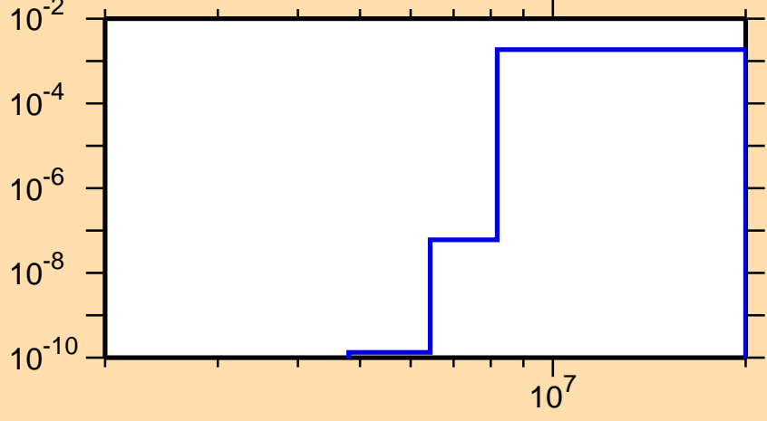
\sigma vs. E for ^{207}\text{Rn}(n,d)
