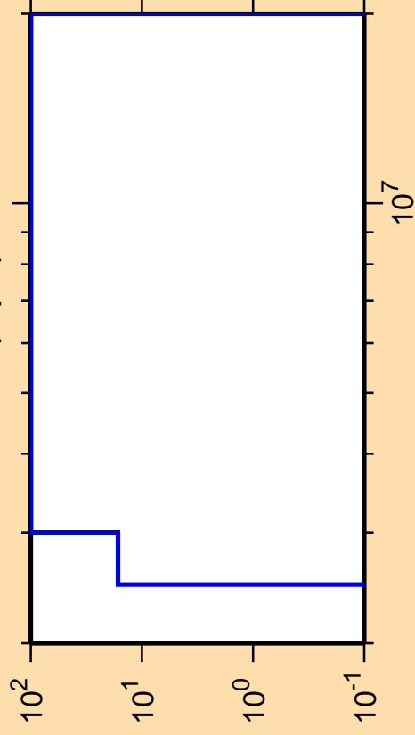
\Delta\sigma/\sigma vs. E for ^{207}\text{Rn}(n,p\alpha)
