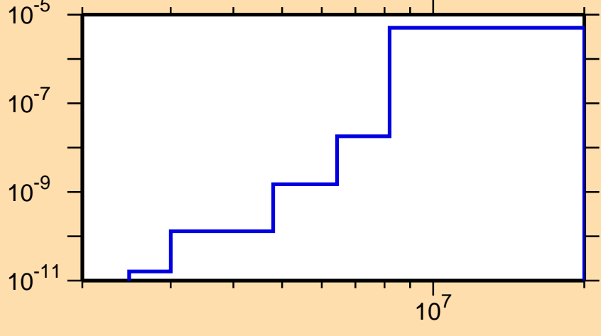
\sigma vs. E for ^{207}\text{Rn}(n,p\alpha)
