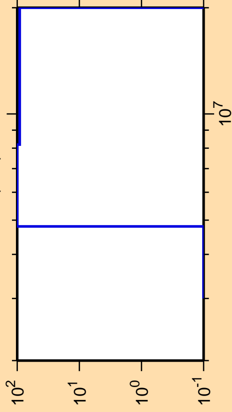
\Delta\sigma/\sigma vs. E for ^{208}\text{Rn}(n,d)
