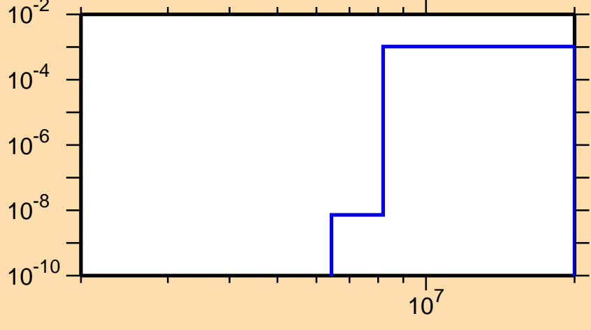
\sigma vs. E for ^{208}\text{Rn}(n,d)
