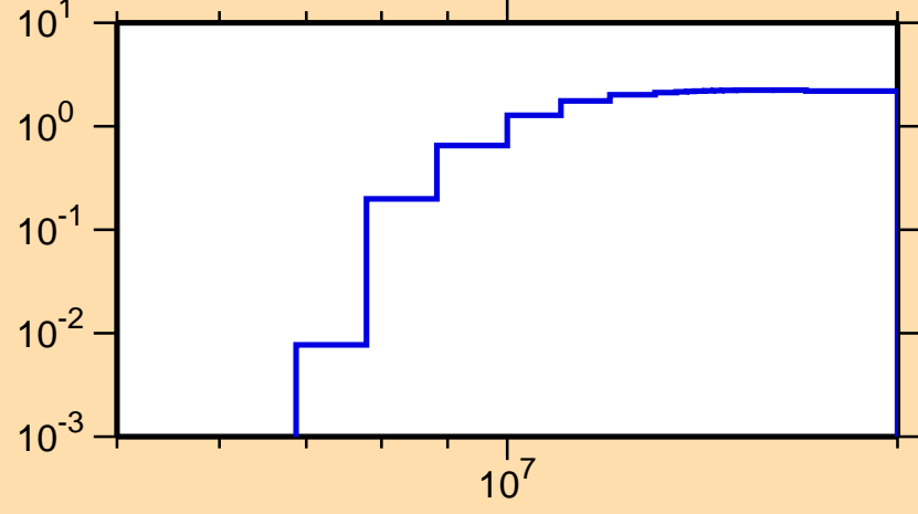
\sigma vs. E for ^{209}\text{Rn}(n,2n)
