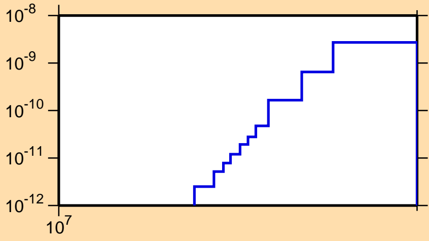
\sigma vs. E for ^{209}\text{Rn}(\text{mt117})
