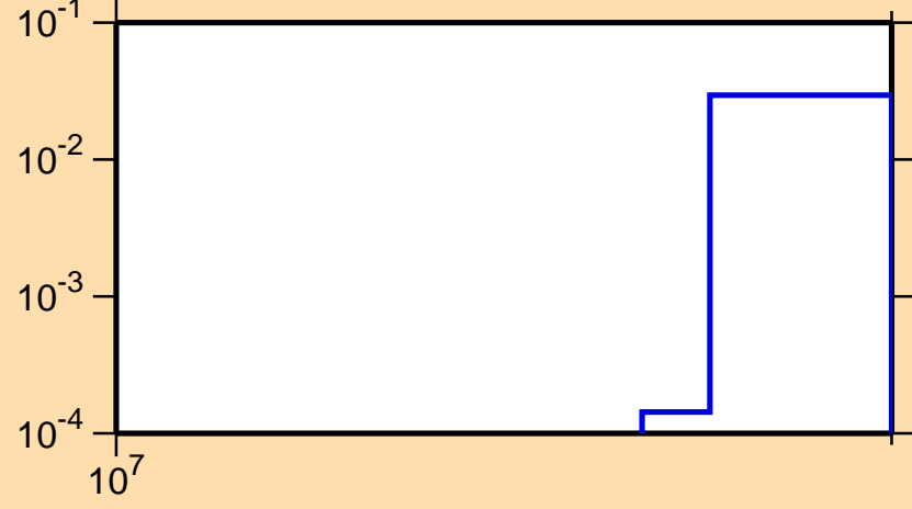
\sigma vs. E for ^{209}\text{Rn}(n,3n)
