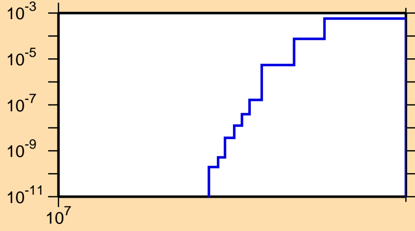
\sigma vs. E for ^{209}\text{Rn}(n,2np)
