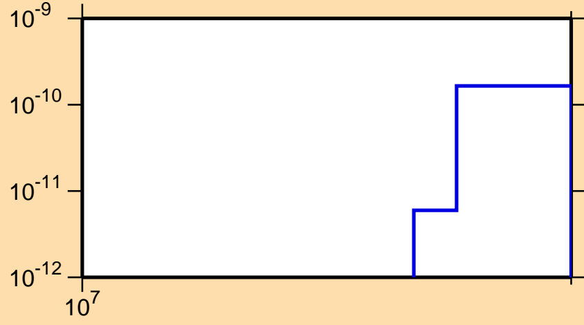
\sigma vs. E for ^{209}\text{Rn} (mt 34)
