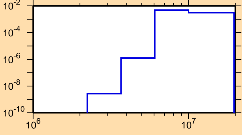
\sigma vs. E for ^{209}\text{Rn}(n,\alpha)
