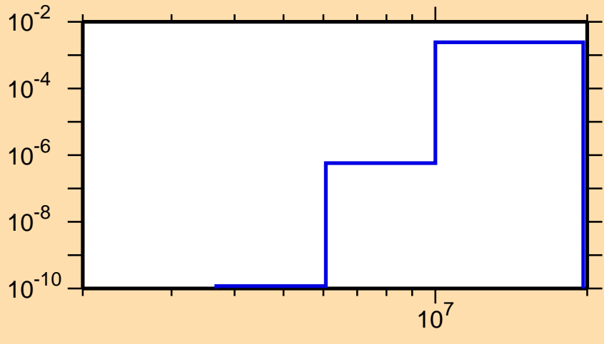
\sigma vs. E for ^{209}\text{Rn}(n,d)
