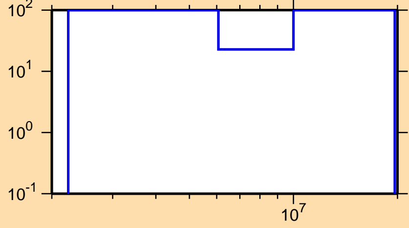
\Delta\sigma/\sigma vs. E for ^{209}\text{Rn}(n,n\text{cont.})
