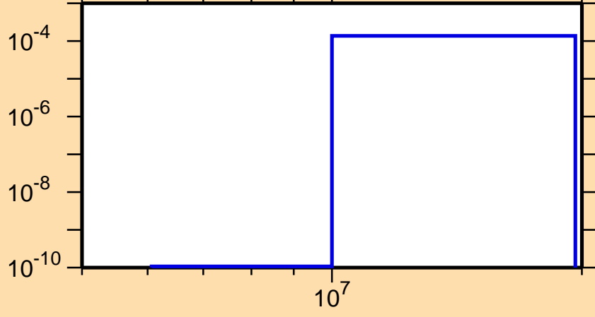
\sigma vs. E for ^{209}\text{Rn}(n,t)
