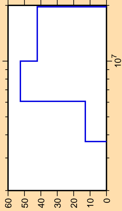
\Delta\sigma/\sigma vs. E for ^{209}\text{Rn}(n,np)
