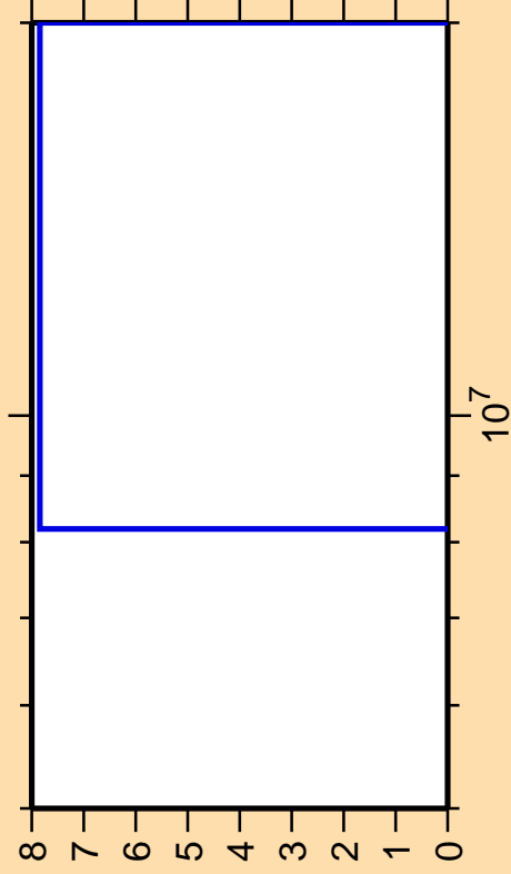
\Delta\sigma/\sigma vs. E for ^{209}\text{Rn}(\text{mt } 34)
