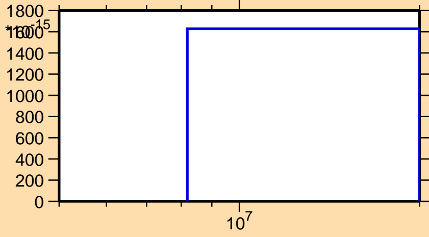
\sigma vs. E for ^{209}\text{Rn}(\text{mt } 34)
