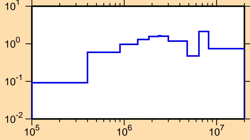
\sigma vs. E for ^{209}\text{Rn}(n,\text{inel.})
