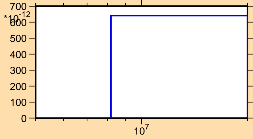
\sigma vs. E for ^{209}\text{Rn}(\text{mt } 45)
