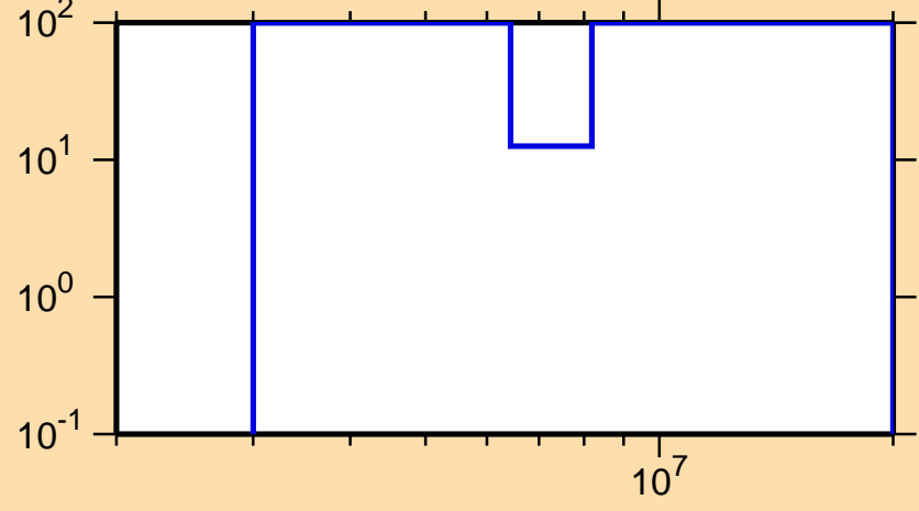
\Delta\sigma/\sigma vs. E for ^{209}\text{Rn}(n,ncont.)
