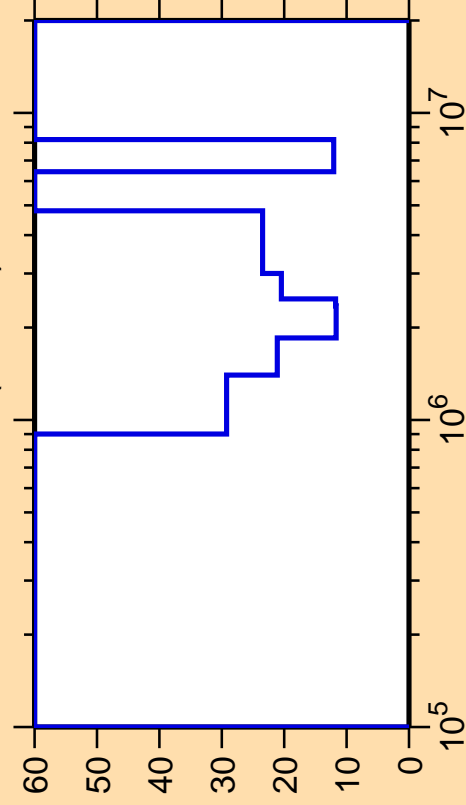
\Delta\sigma/\sigma vs. E for ^{209}\text{Rn}(n,\text{inel.})
