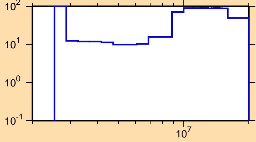
\Delta\sigma/\sigma vs. E for ^{211}\text{Rn}(n,n\text{cont.})
