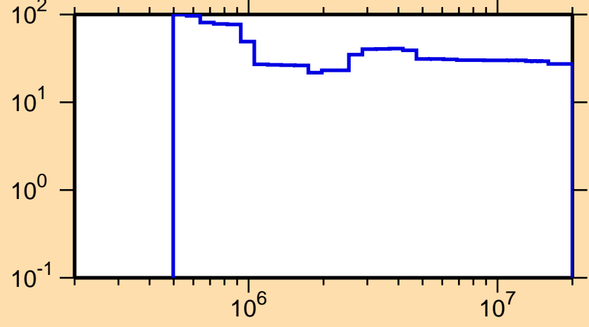
\Delta\sigma/\sigma vs. E for ^{211}\text{Rn}(n,n_1)
