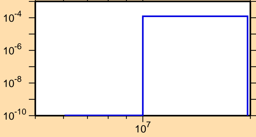
\sigma vs. E for ^{211}\text{Rn}(n,t)
