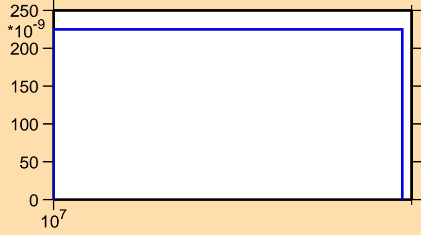
\sigma vs. E for ^{211}\text{Rn}(n,nd)
