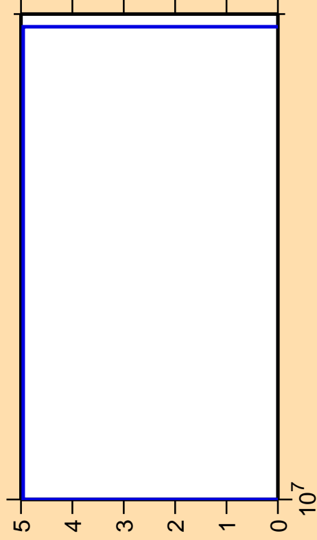
\Delta\sigma/\sigma vs. E for ^{211}\text{Rn} (mt 34)
