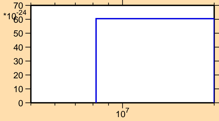
\sigma vs. E for ^{211}\text{Rn}(\text{mt } 42)
