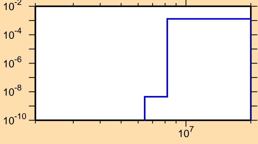
\sigma vs. E for ^{211}\text{Rn}(n,d)
