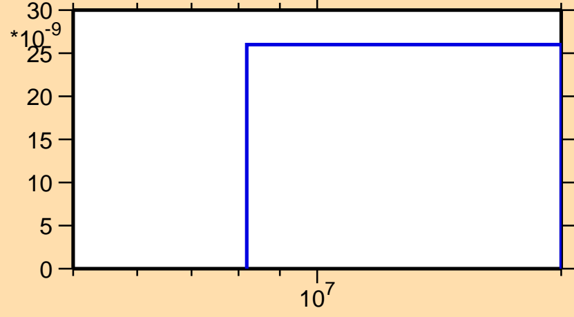
\sigma vs. E for ^{211}\text{Rn}(n,\text{He}3)
