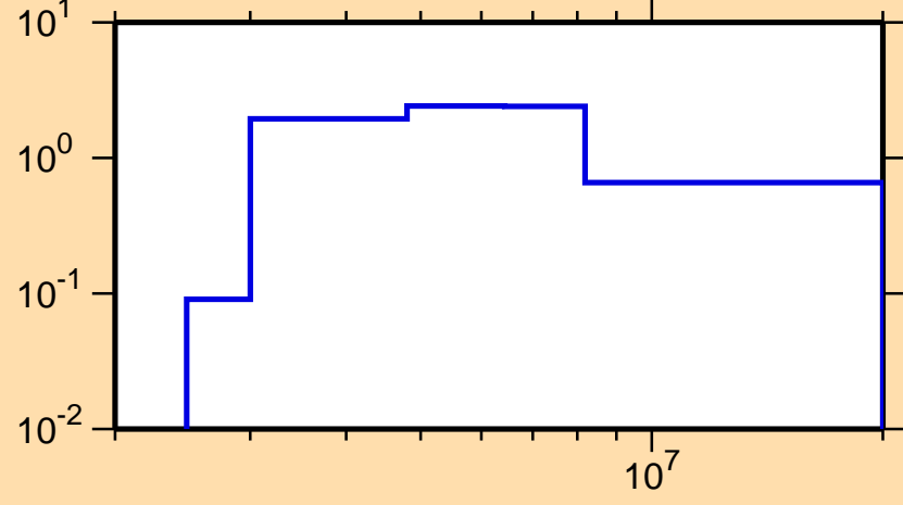
\sigma vs. E for ^{211}\text{Rn}(n,n\text{cont.})
