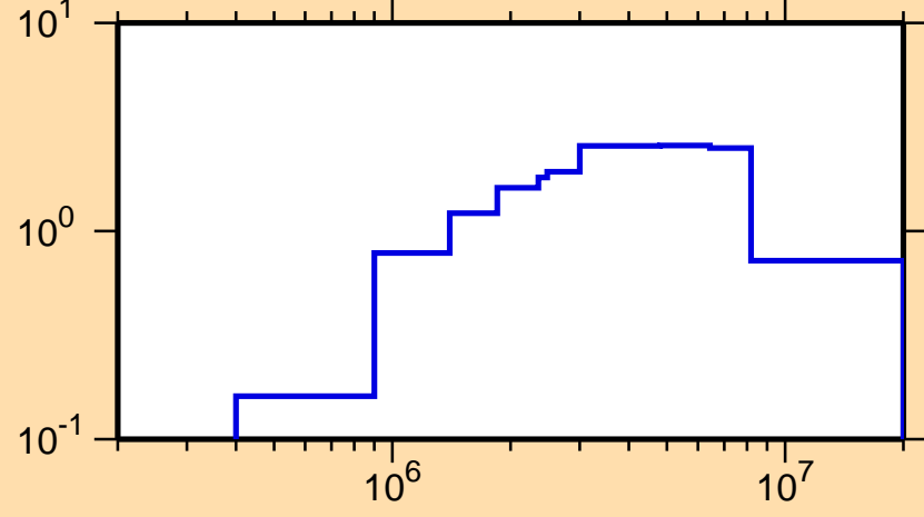
\sigma vs. E for ^{211}\text{Rn}(n,\text{inel.})
