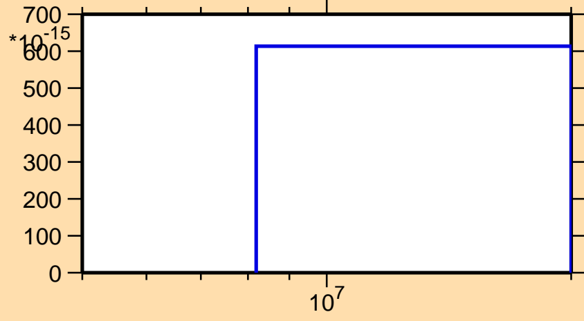
\sigma vs. E for ^{211}\text{Rn}(\text{mt } 34)
