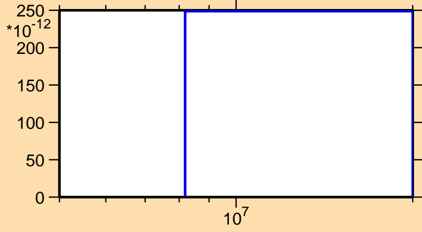
\sigma vs. E for ^{211}\text{Rn}(\text{mt } 45)
