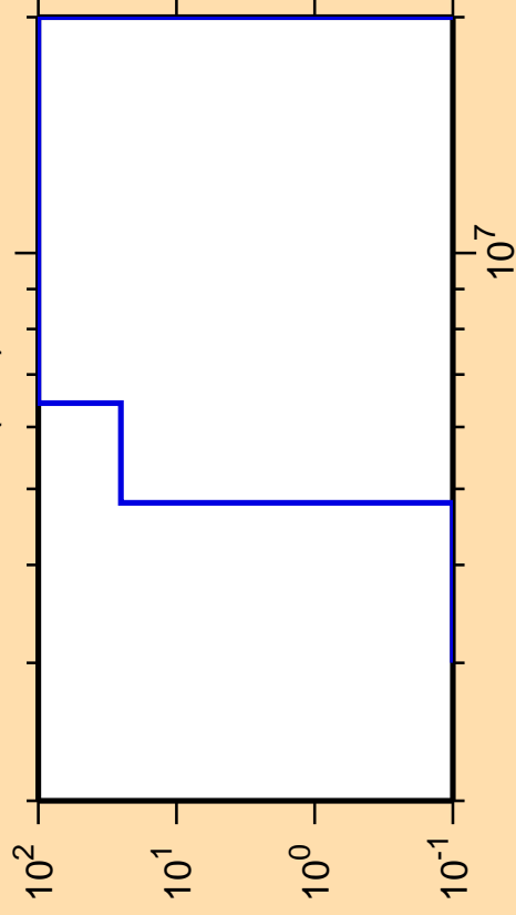
\Delta\sigma/\sigma vs. E for ^{211}\text{Rn}(n,d)
