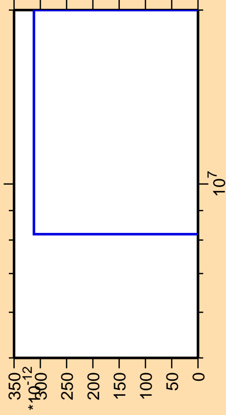
\Delta\sigma/\sigma vs. E for ^{211}\text{Rn}(\text{mt } 42)
