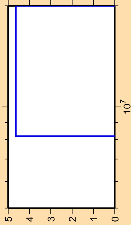
\Delta\sigma/\sigma vs. E for ^{211}\text{Rn}(\text{mt } 34)
