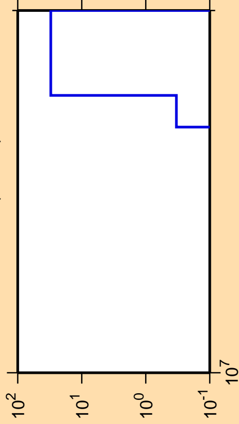
\Delta\sigma/\sigma vs. E for ^{212}\text{Rn} (mt 34)
