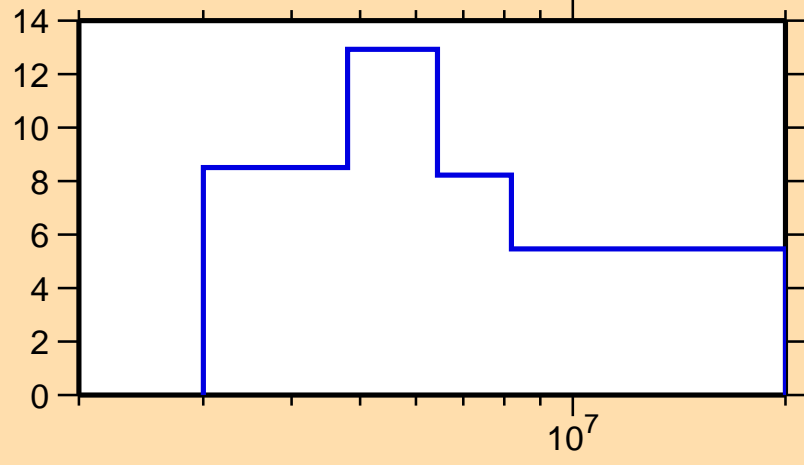
\Delta\sigma/\sigma vs. E for ^{212}\text{Rn}(n, el.)
