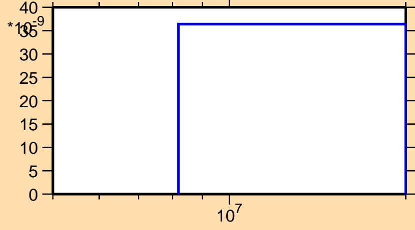
\sigma vs. E for ^{212}\text{Rn}(n,nd)
