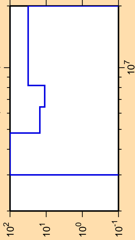
\Delta\sigma/\sigma vs. E for ^{212}\text{Rn}(n, ncont.)
