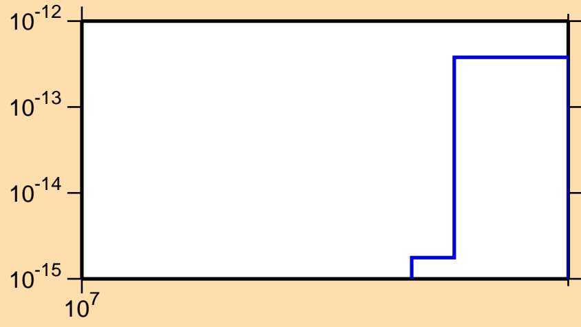
\sigma vs. E for ^{219}\text{Rn}(\text{mt } 34)
