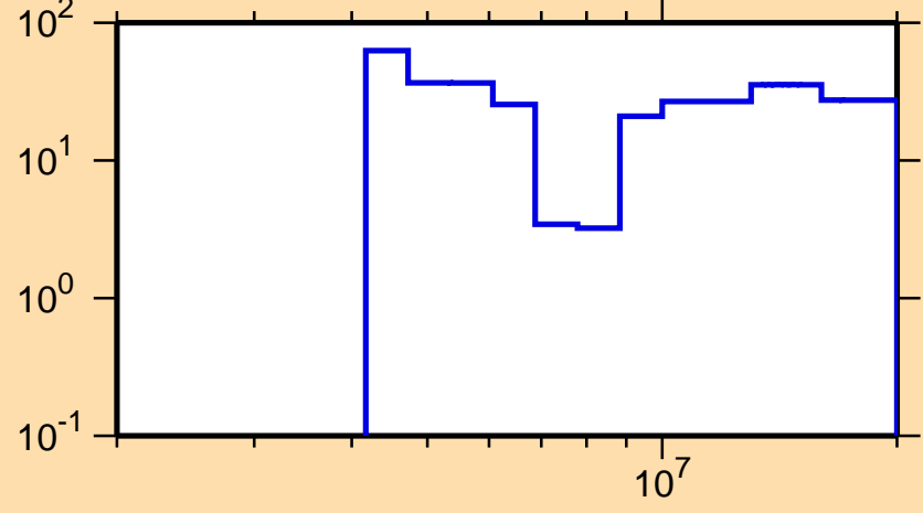
\Delta\sigma/\sigma vs. E for ^{219}\text{Rn}(n,2n)
