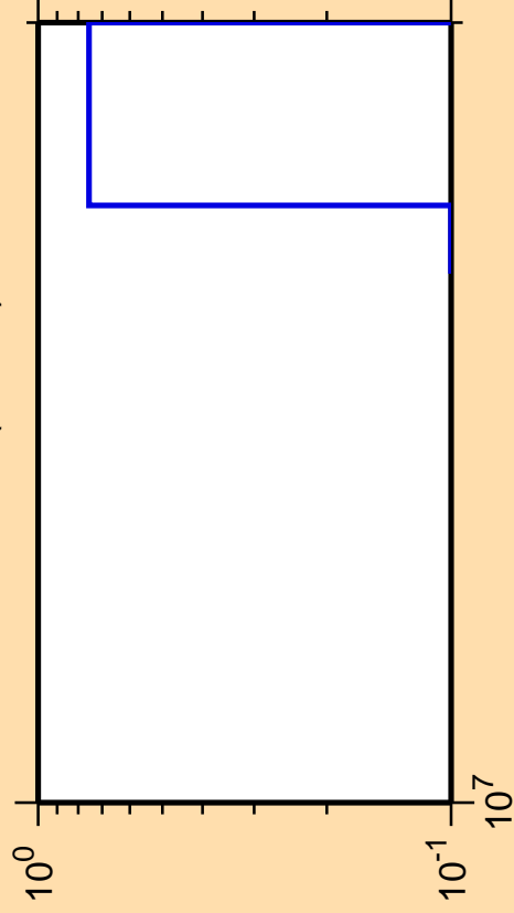
\Delta\sigma/\sigma vs. E for ^{219}\text{Rn} (mt 42)
