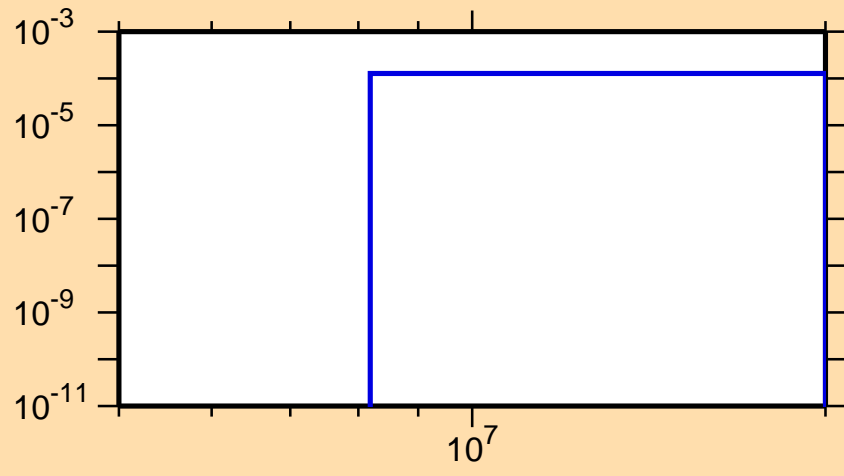
\sigma vs. E for ^{219}\text{Rn}(n,t)
