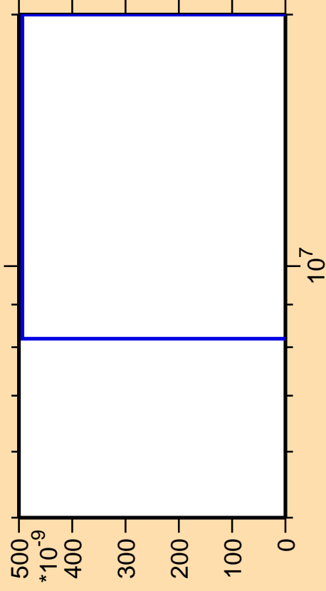
\Delta\sigma/\sigma vs. E for ^{219}\text{Rn}(\text{mt } 34)
