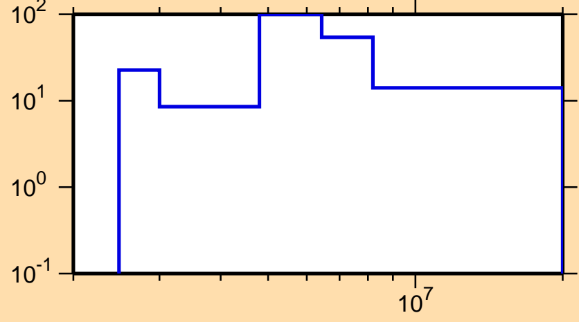
\Delta\sigma/\sigma vs. E for ^{219}\text{Rn}(n,\gamma)
