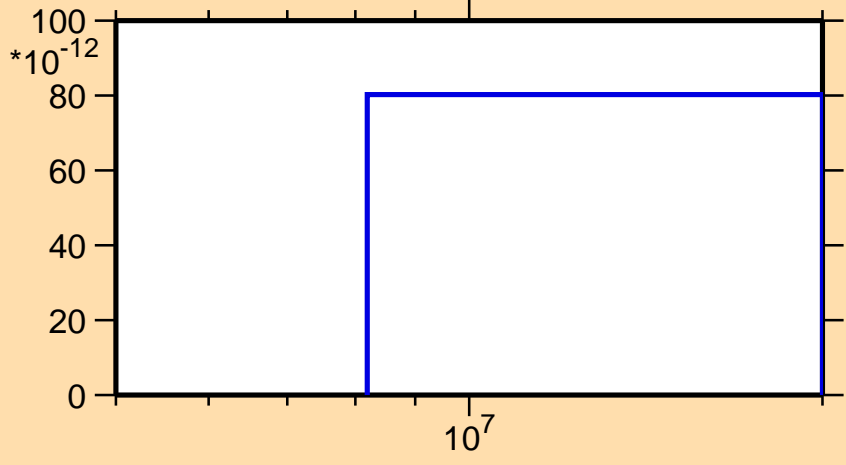
\sigma vs. E for ^{219}\text{Rn} (mt 45)
