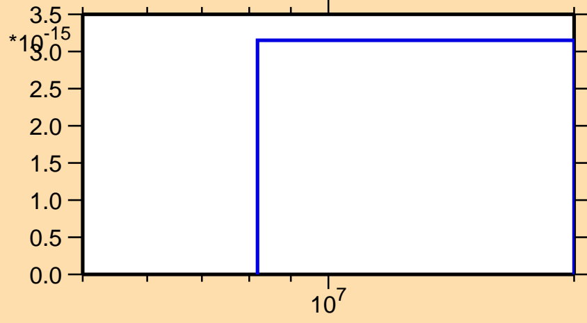
\sigma vs. E for ^{219}\text{Rn}(\text{mt } 34)
