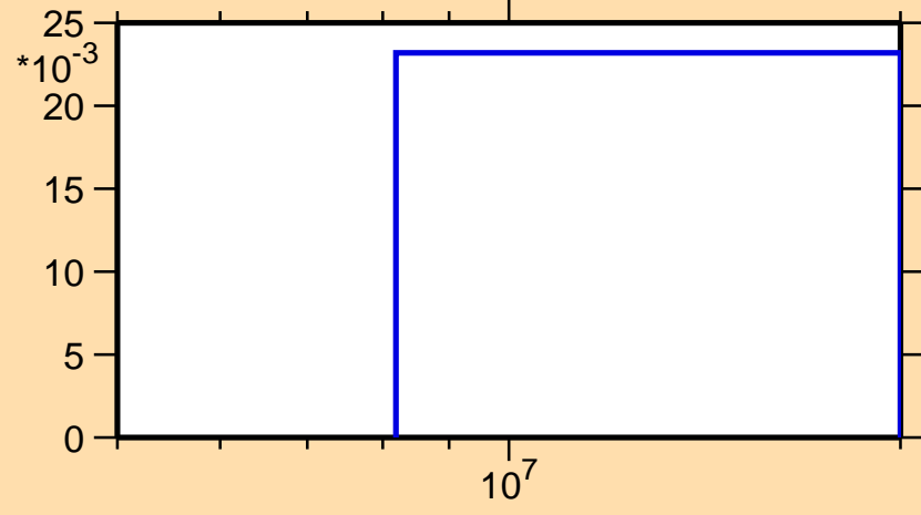
\sigma vs. E for ^{219}\text{Rn}(n,3n\alpha)
