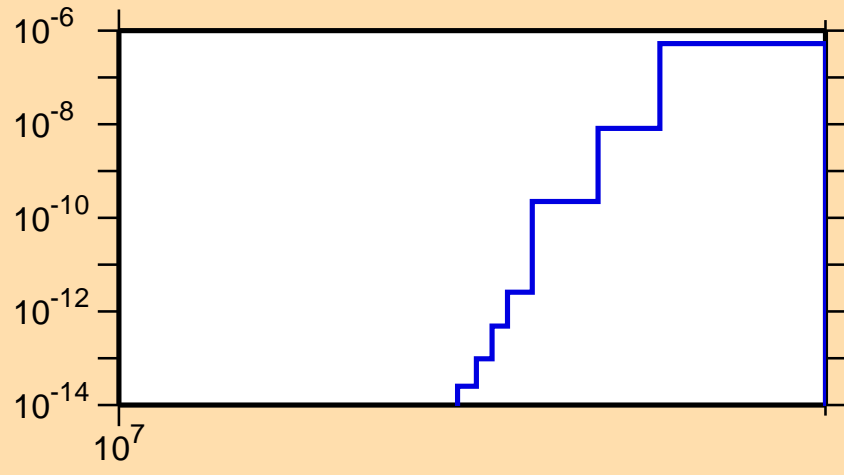
\sigma vs. E for ^{220}\text{Rn}(n,\text{nd})
