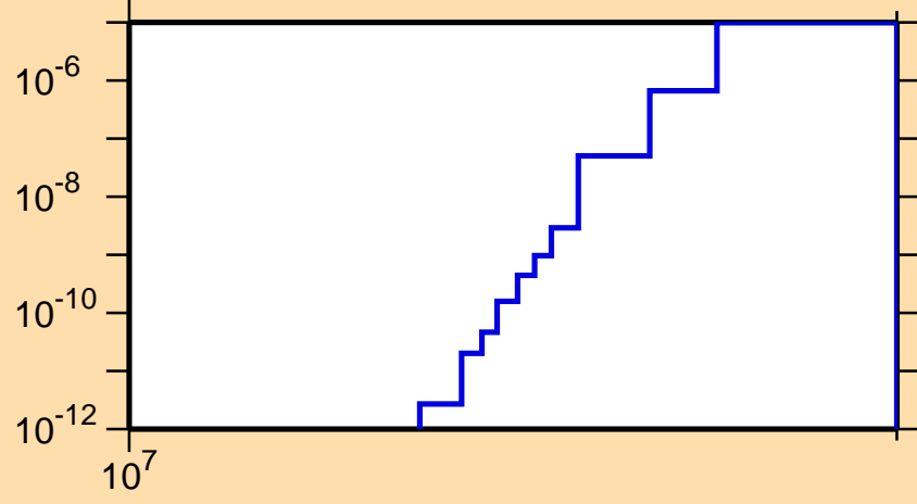
\sigma vs. E for ^{220}\text{Rn}(n,nt)
