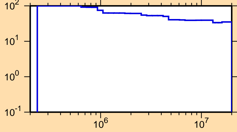
\Delta\sigma/\sigma vs. E for ^{220}\text{Rn}(n,\text{nonel.})
