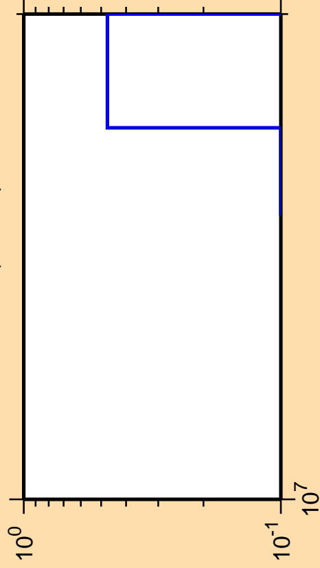
\Delta\sigma/\sigma vs. E for ^{220}\text{Rn}(\text{mt 11})
