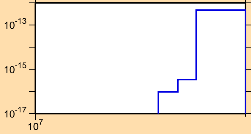
\sigma vs. E for ^{220}\text{Rn}(\text{mt 11})
