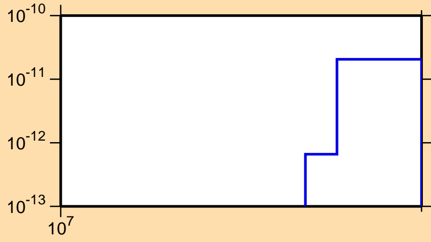
\sigma vs. E for ^{220}\text{Rn}(n,\text{He}3)
