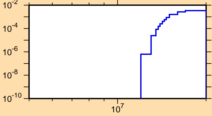
\sigma vs. E for ^{220}\text{Rn}(n,3n\alpha)
