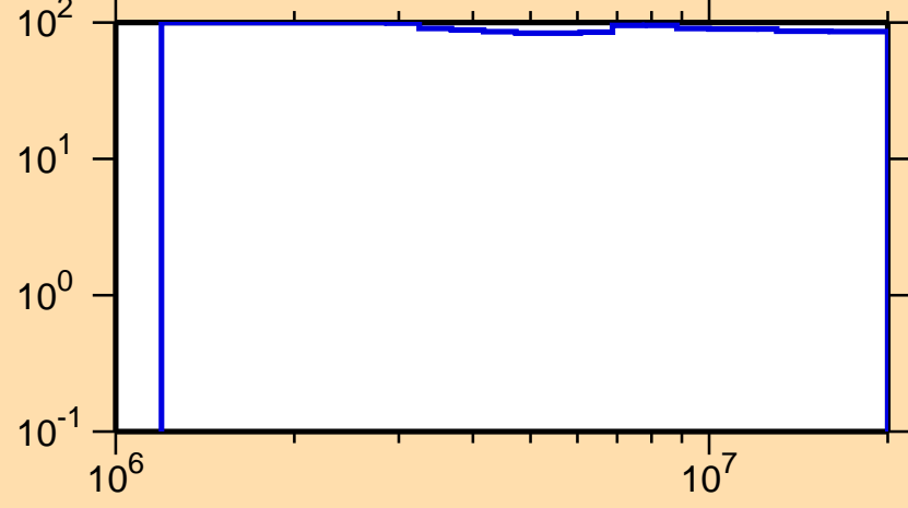
\Delta\sigma/\sigma vs. E for ^{220}\text{Rn}(n,n\text{cont.})
