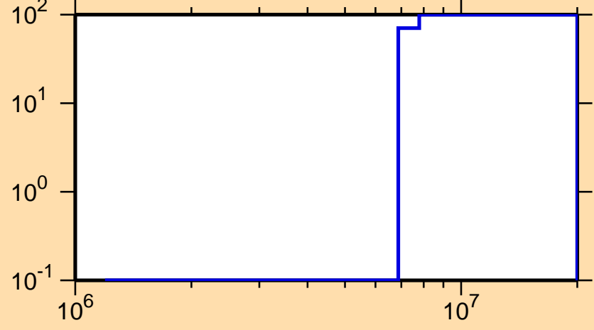
\Delta\sigma/\sigma vs. E for ^{220}\text{Rn}(n,f)
