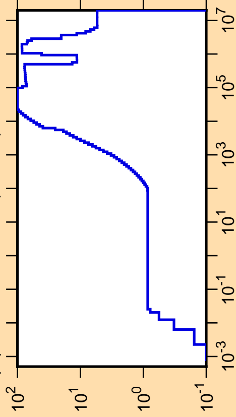
\Delta\mu/\mu vs. E for ^{221}\text{Rn}(\text{mt251})
