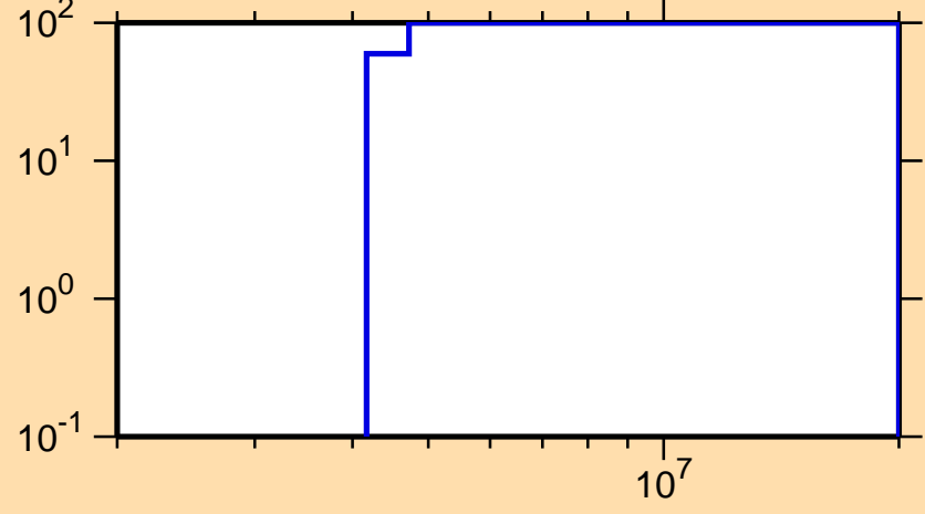
\Delta\sigma/\sigma vs. E for ^{221}\text{Rn}(n,n\text{cont.})
