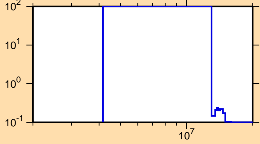
\Delta\sigma/\sigma vs. E for ^{221}\text{Rn}(n,n_1)
