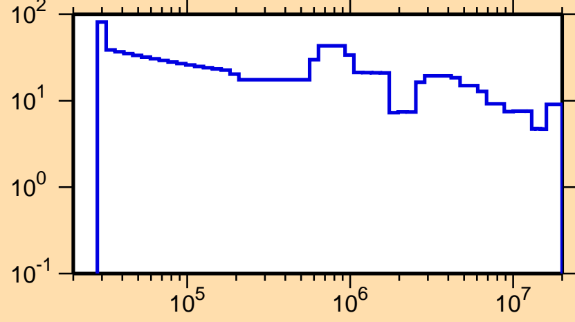
\Delta\sigma/\sigma vs. E for ^{221}\text{Rn}(n,\text{tot.})
