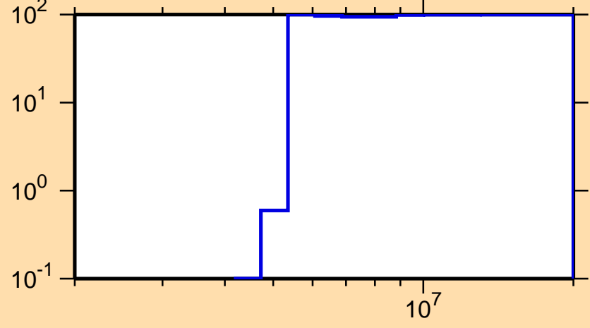
\Delta\sigma/\sigma vs. E for ^{221}\text{Rn}(n,f)
