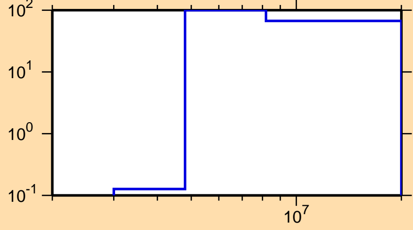
\Delta\sigma/\sigma vs. E for ^{221}\text{Rn}(n,p)
