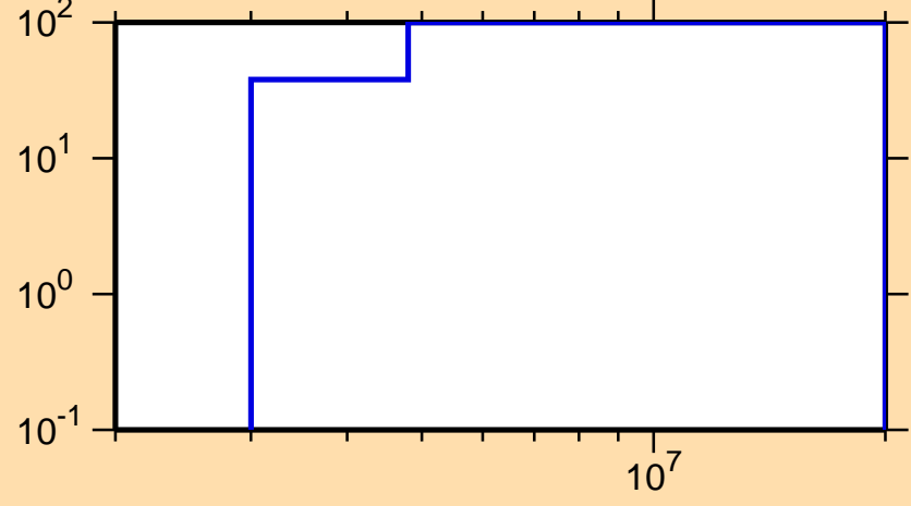
\Delta\sigma/\sigma vs. E for ^{221}\text{Rn}(n,ncont.)
