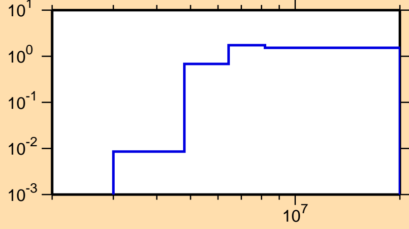
\sigma vs. E for ^{221}\text{Rn}(n,2n)
