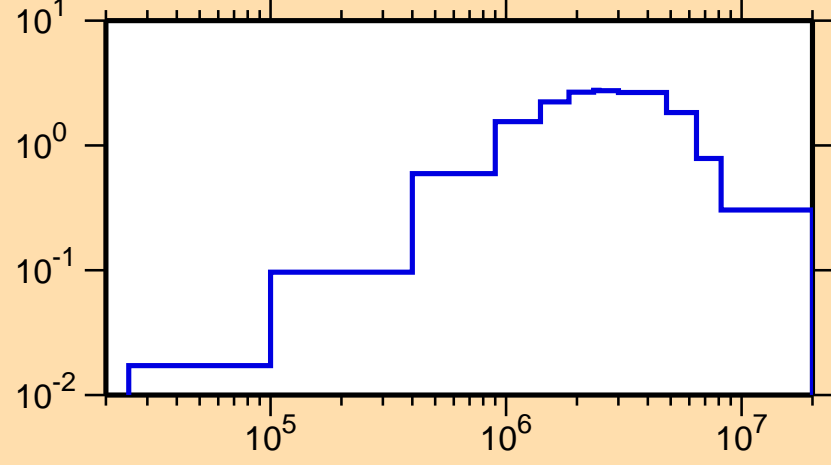
\sigma vs. E for ^{221}\text{Rn}(n,\text{inel.})
