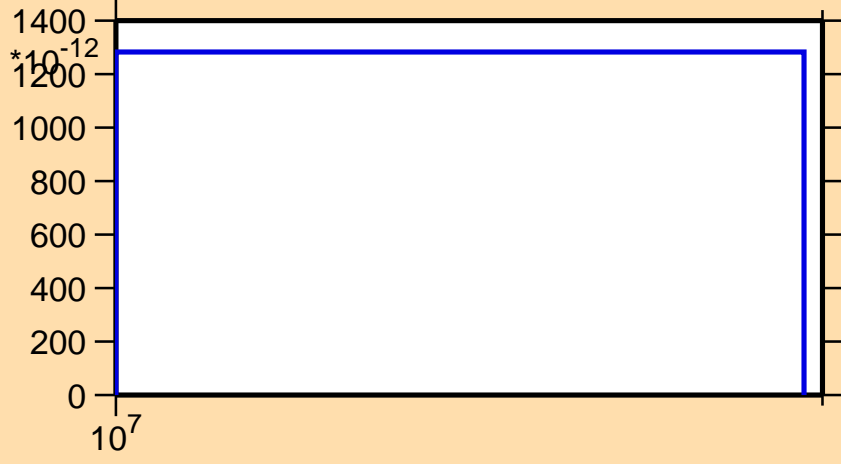
\sigma vs. E for ^{222}\text{Rn}(n,\text{nd})
