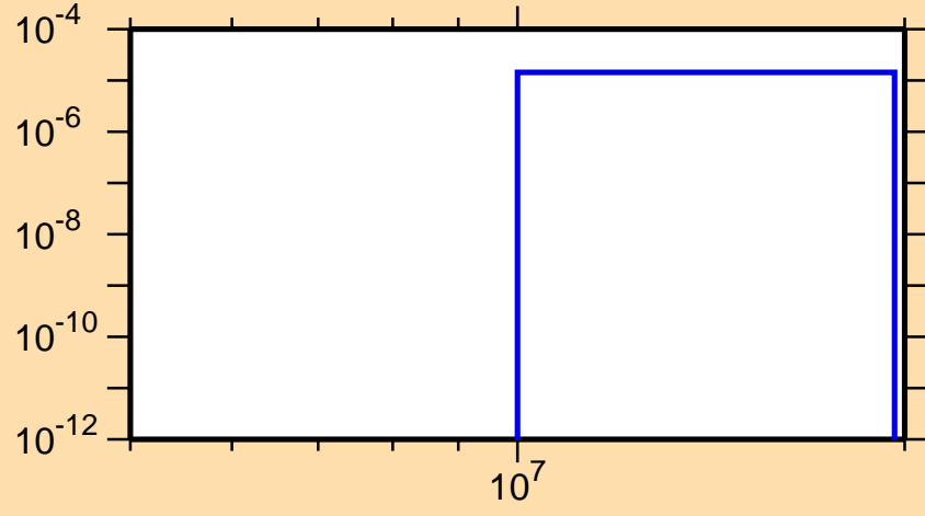
\sigma vs. E for ^{222}\text{Rn}(n,np)
