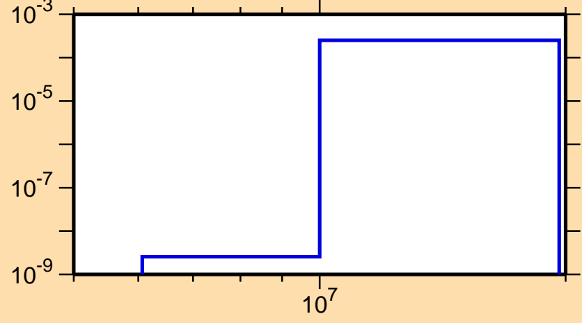
\sigma vs. E for ^{222}\text{Rn}(n,p)
