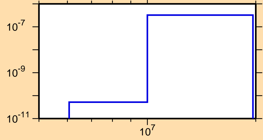
\sigma vs. E for ^{222}\text{Rn}(n,2n\alpha)
