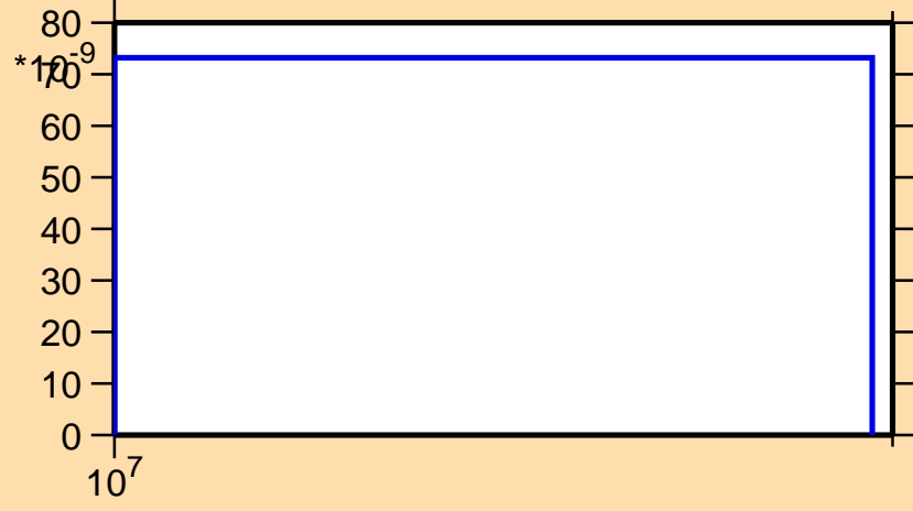
\sigma vs. E for ^{222}\text{Rn}(n,nt)
