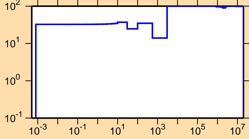
\Delta\sigma/\sigma vs. E for ^{222}\text{Rn}(n,\gamma)
