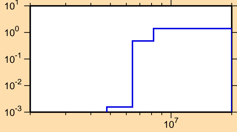
\sigma vs. E for ^{222}\text{Rn}(n,2n)
