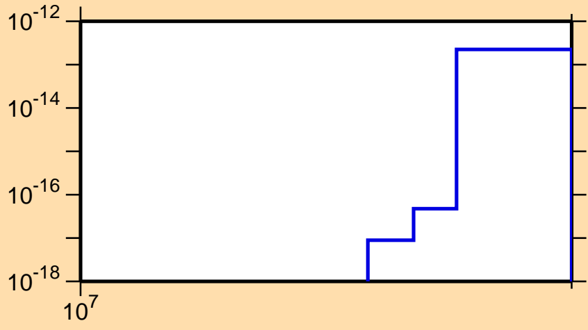
\sigma vs. E for ^{223}\text{Rn}(\text{mt } 11)
