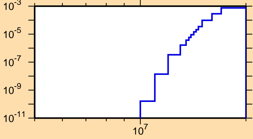
\sigma vs. E for ^{223}\text{Rn}(n,d)
