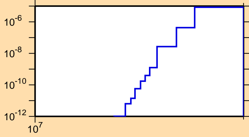
\sigma vs. E for ^{223}\text{Rn}(n,nt)
