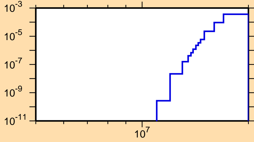
\sigma vs. E for ^{223}\text{Rn}(n,np)
