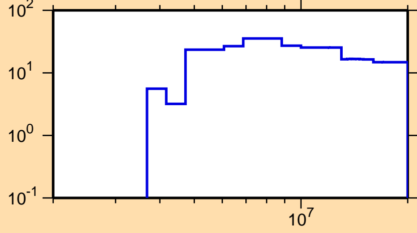
\Delta\sigma/\sigma vs. E for ^{223}\text{Rn}(n,\text{tot.})
