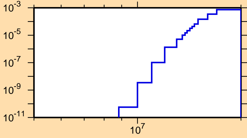
\sigma vs. E for ^{223}\text{Rn}(n,t)
