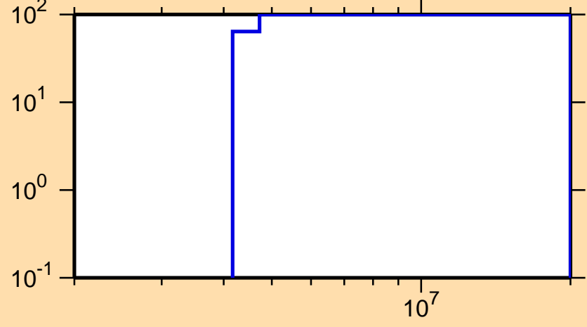
\Delta\sigma/\sigma vs. E for ^{223}\text{Rn}(n,ncont.)
