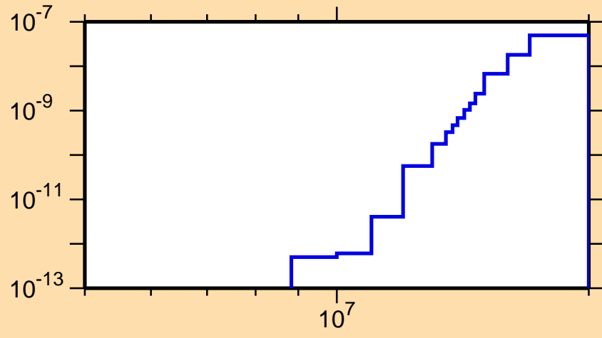
\sigma vs. E for ^{223}\text{Rn}(n,3n\alpha)
