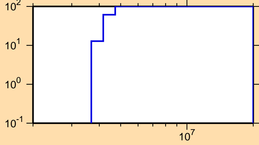
\Delta\sigma/\sigma vs. E for ^{223}\text{Rn}(n,\text{inel.})
