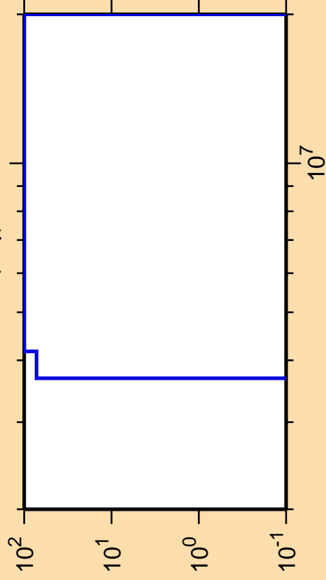
\Delta\sigma/\sigma vs. E for ^{223}\text{Rn}(n,\gamma)
