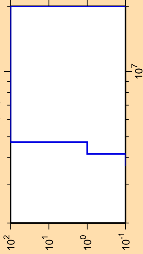
\Delta\sigma/\sigma vs. E for ^{223}\text{Rn}(n,f)
