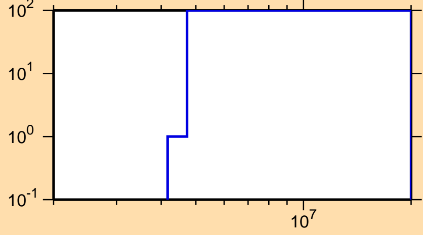
\Delta\sigma/\sigma vs. E for ^{223}\text{Rn}(n,f)
