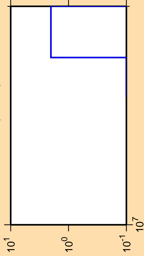
\Delta\sigma/\sigma vs. E for ^{223}\text{Rn}(\text{mt } 11)
