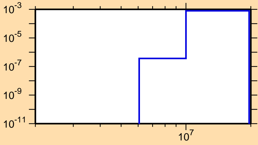
\sigma vs. E for ^{223}\text{Rn}(n,p)
