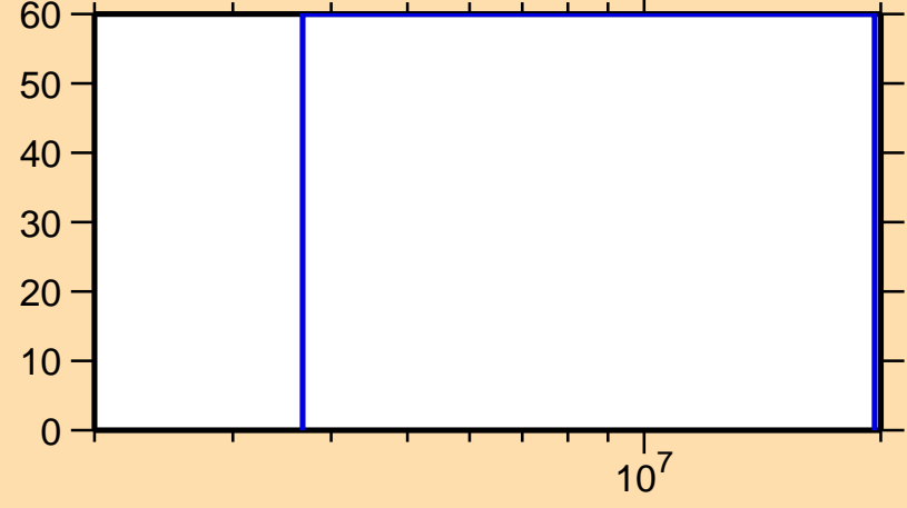
\Delta\sigma/\sigma vs. E for ^{223}\text{Rn}(n,ncont.)
