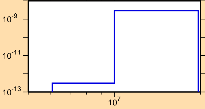
\sigma vs. E for ^{223}\text{Rn}(n,3n\alpha)
