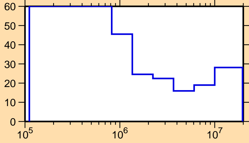
\Delta\sigma/\sigma vs. E for ^{223}\text{Rn}(n,n\text{onel.})
