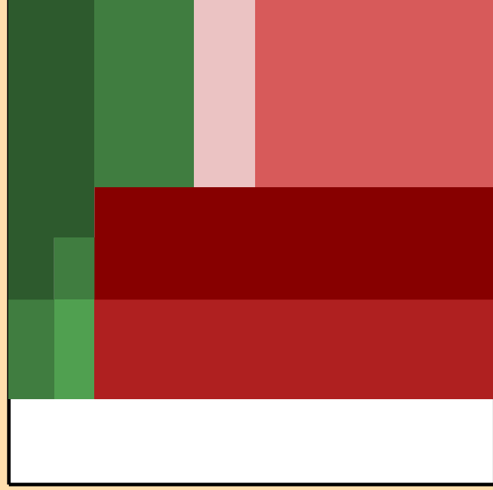
\Delta\sigma/\sigma vs. E for ^{223}\text{Rn}(n,\text{inel.})
