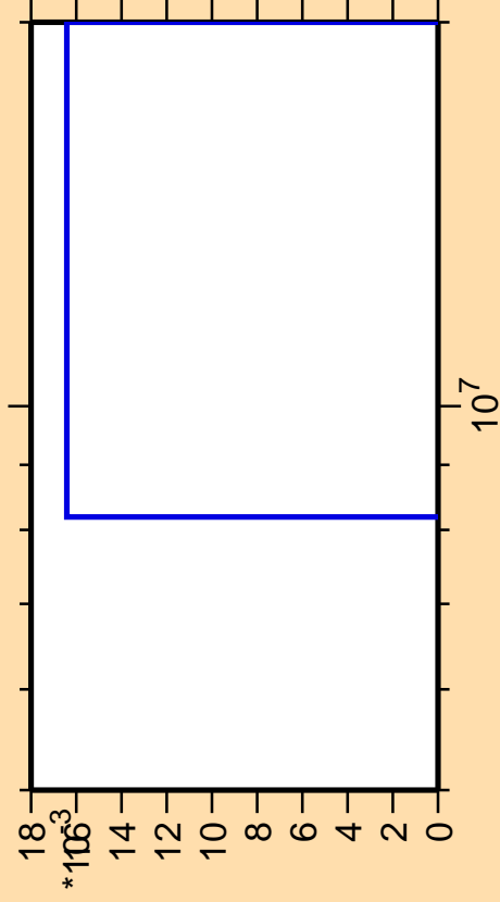
\Delta\sigma/\sigma vs. E for ^{223}\text{Rn}(\text{mt } 11)
