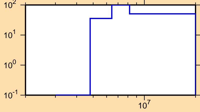
\Delta\sigma/\sigma vs. E for ^{223}\text{Rn}(n,p)
