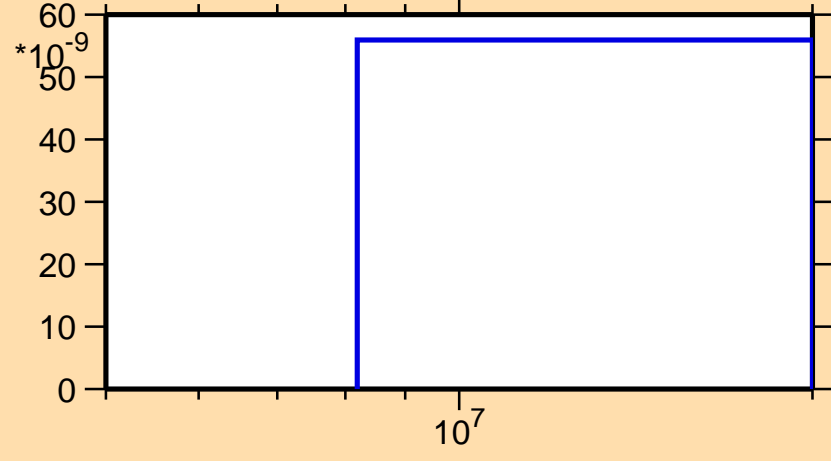
\sigma vs. E for ^{223}\text{Rn}(n,nd)
