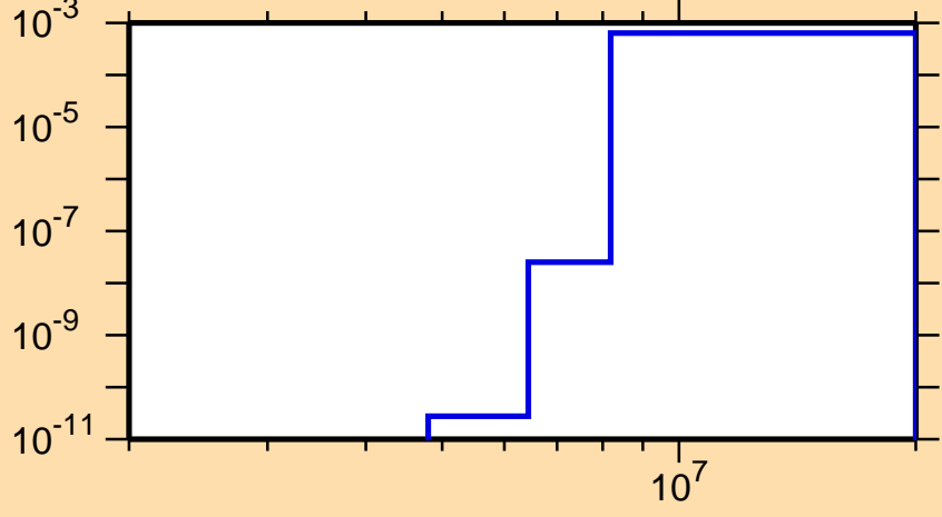
\sigma vs. E for ^{223}\text{Rn}(n,p)
