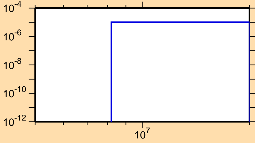
\sigma vs. E for ^{223}\text{Rn}(n,np)
