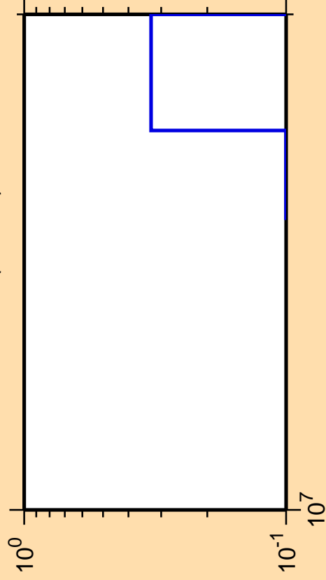
\Delta\sigma/\sigma vs. E for ^{224}\text{Rn}(\text{mt 11})
