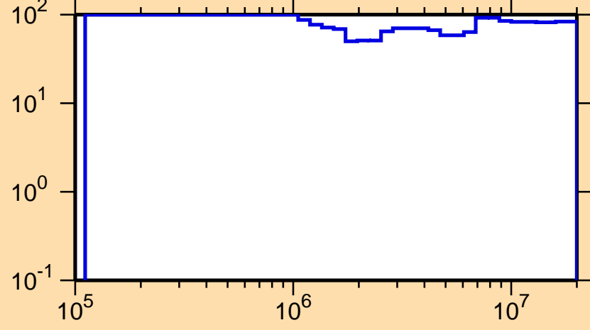
\Delta\sigma/\sigma vs. E for ^{224}\text{Rn}(n,n\text{cont.})
