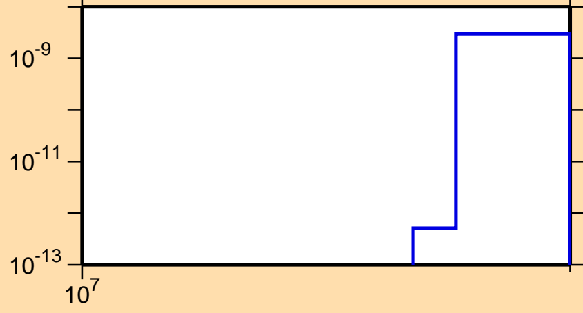
\sigma vs. E for ^{224}\text{Rn}(n,2np)
