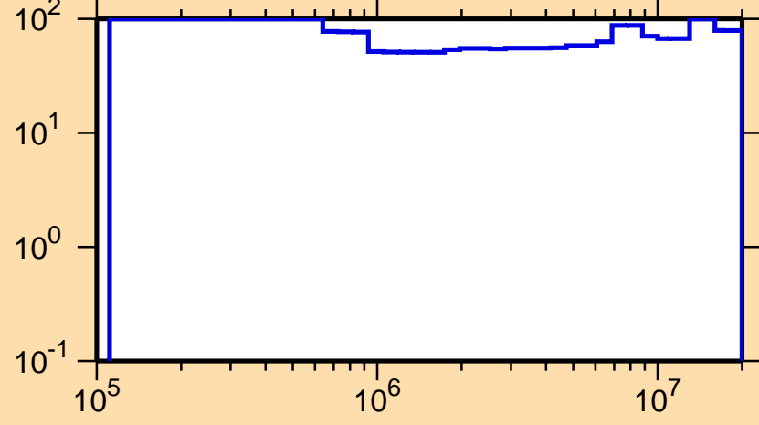
\Delta\sigma/\sigma vs. E for ^{224}\text{Rn}(n,\text{inel.})
