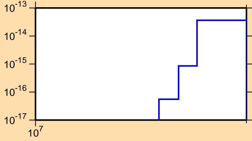
\sigma vs. E for ^{224}\text{Rn}(\text{mt 11})
