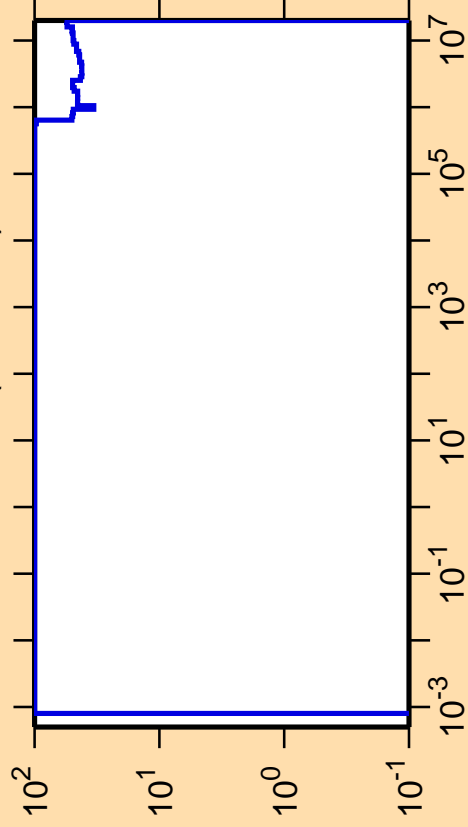
\Delta\sigma/\sigma vs. E for ^{224}\text{Rn}(n,\text{nonel.})
