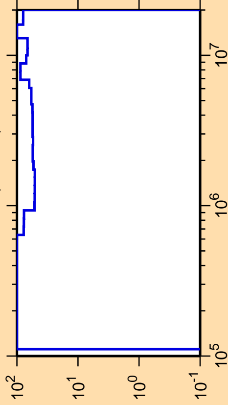
\Delta\sigma/\sigma vs. E for ^{224}\text{Rn}(n,\text{inel.})
