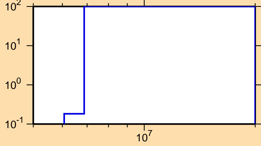
\Delta\sigma/\sigma vs. E for ^{224}\text{Rn}(n,f)
