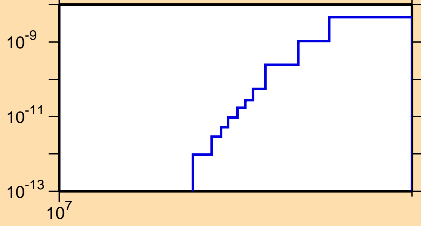
\sigma vs. E for ^{224}\text{Rn}(n,3n\alpha)
