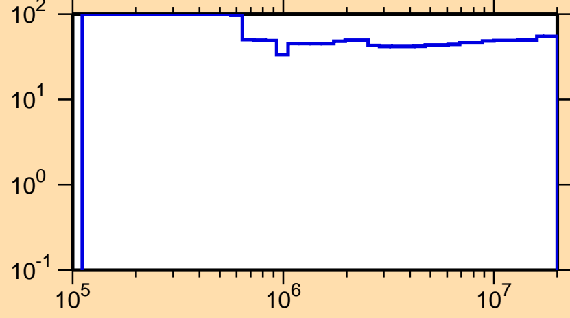
\Delta\sigma/\sigma vs. E for ^{224}\text{Rn}(n,\text{nonel.})
