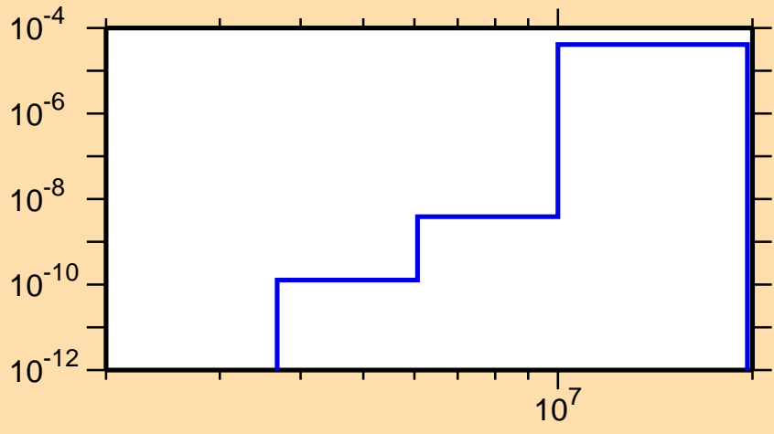
\sigma vs. E for ^{224}\text{Rn}(n,n\alpha)
