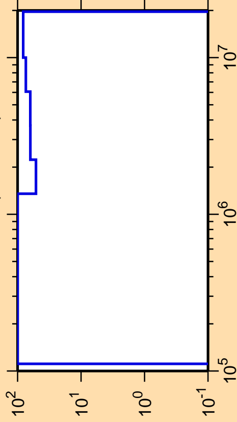
\Delta\sigma/\sigma vs. E for ^{224}\text{Rn}(n,\text{ncont.})
