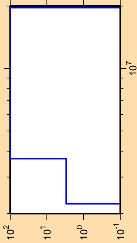
\Delta\sigma/\sigma vs. E for ^{224}\text{Rn}(n,n\alpha)
