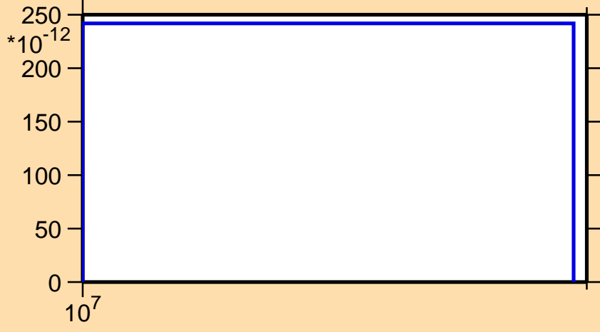
\sigma vs. E for ^{224}\text{Rn}(n,\text{nd})
