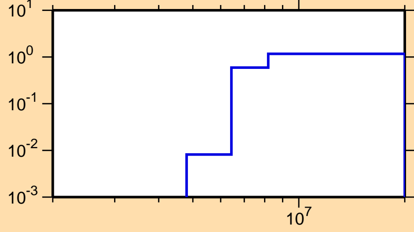
\sigma vs. E for ^{224}\text{Rn}(n,2n)
