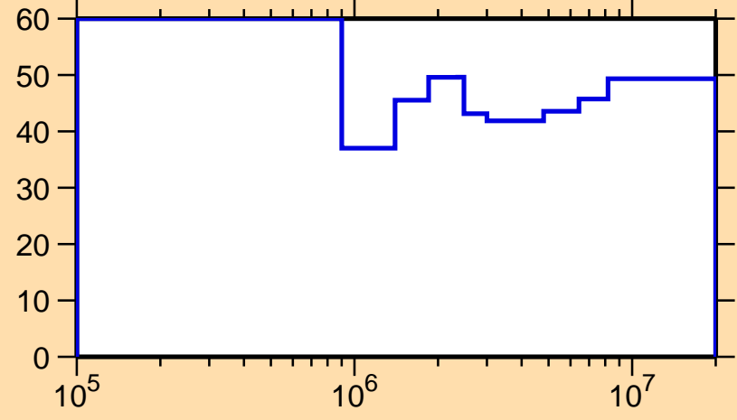
\Delta\sigma/\sigma vs. E for ^{224}\text{Rn}(n,n\text{onel.})
