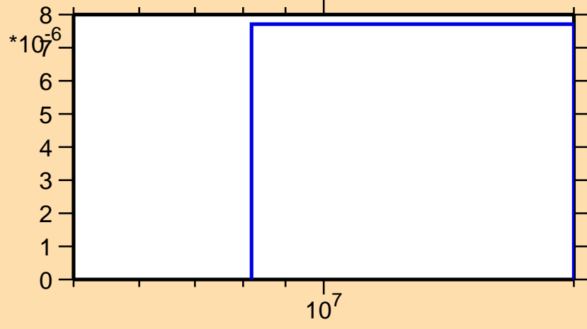
\sigma vs. E for ^{224}\text{Rn}(n,d)
