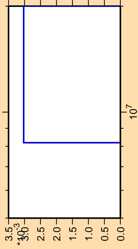
\Delta\sigma/\sigma vs. E for ^{224}\text{Rn}(\text{mt } 11)
