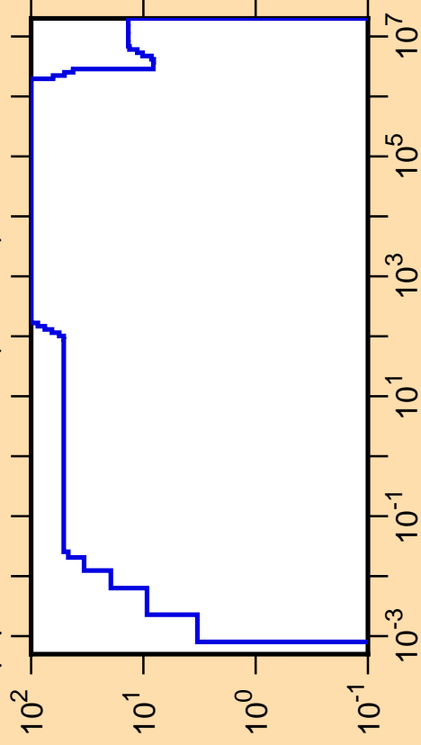
\Delta\mu/\mu vs. E for ^{226}\text{Rn}(\text{mt251})
