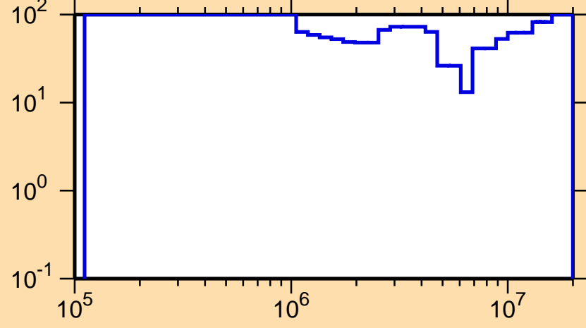
\Delta\sigma/\sigma vs. E for ^{226}\text{Rn}(n,\text{inel.})
