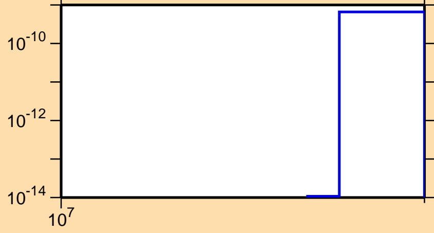
\sigma vs. E for ^{226}\text{Rn}(n,2np)
