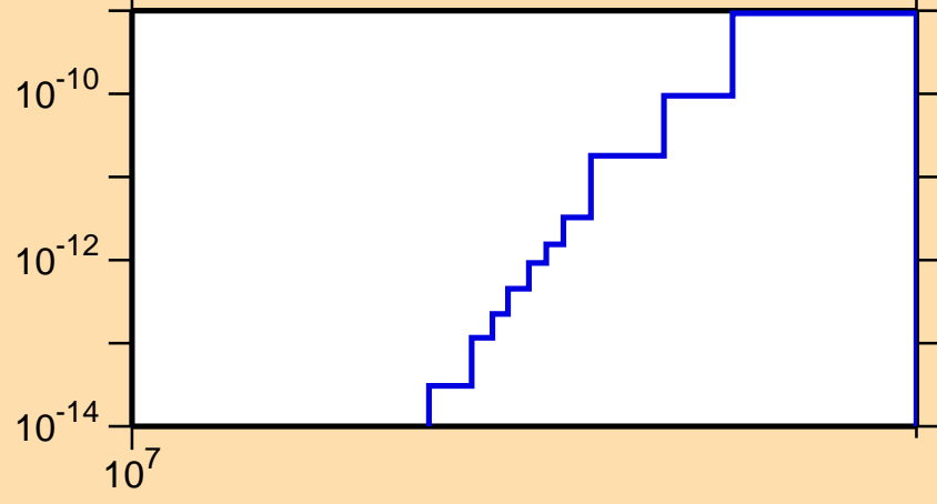
\sigma vs. E for ^{226}\text{Rn}(n,3n\alpha)
