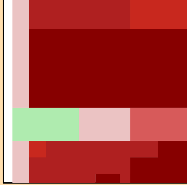
\Delta\sigma/\sigma vs. E for ^{226}\text{Rn}(n,2n)
