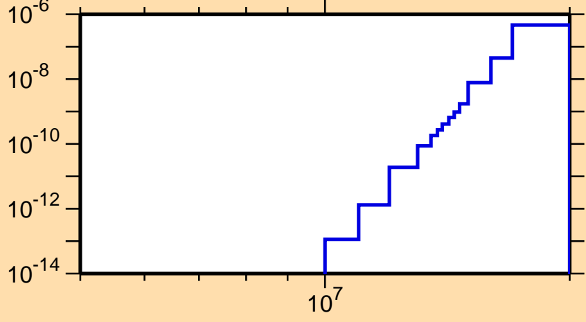
\sigma vs. E for ^{226}\text{Rn}(n,2n\alpha)
