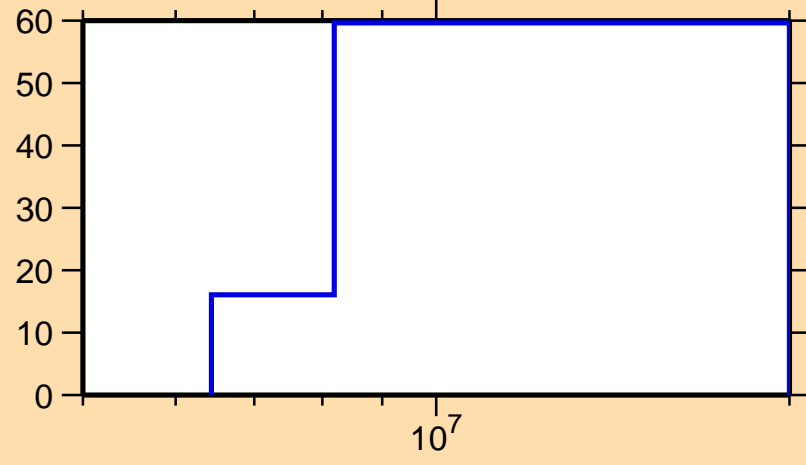
\Delta\sigma/\sigma vs. E for ^{226}\text{Rn}(n,ncont.)
