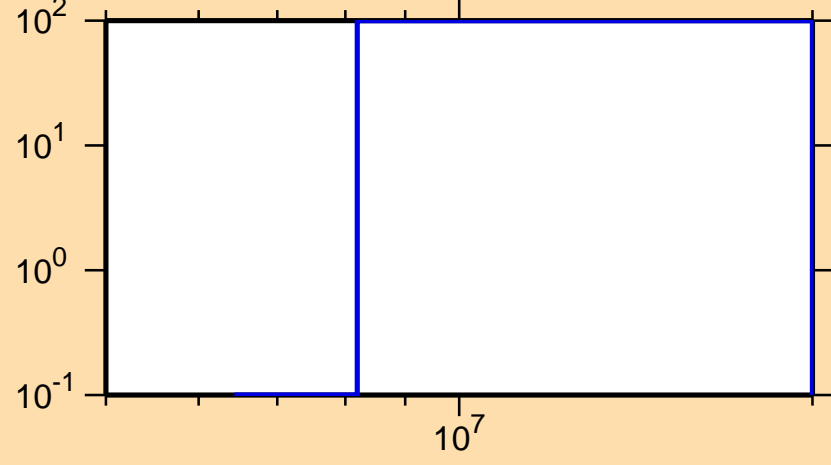
\Delta\sigma/\sigma vs. E for ^{226}\text{Rn}(n,p)
