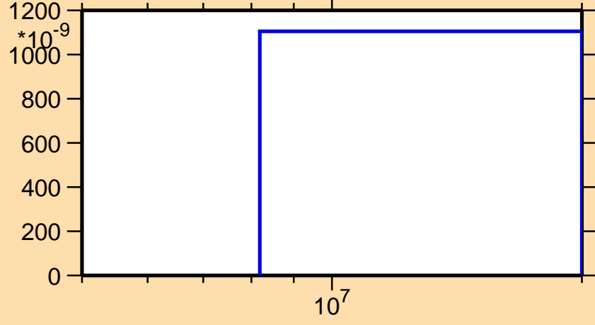
\sigma vs. E for ^{226}\text{Rn}(n,np)
