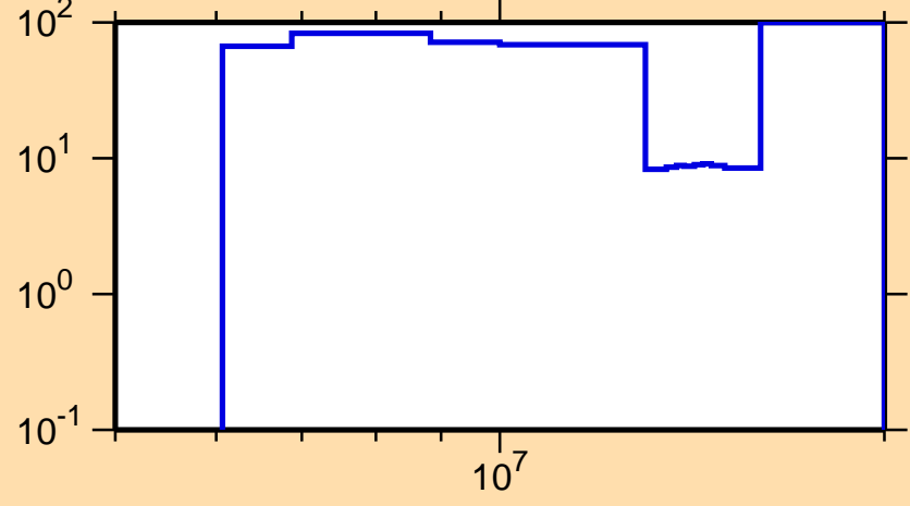
\Delta\sigma/\sigma vs. E for ^{227}\text{Rn}(n,2n)
