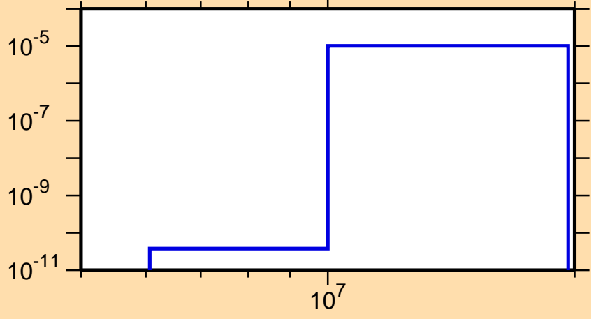
\sigma vs. E for ^{227}\text{Rn}(n,n\alpha)
