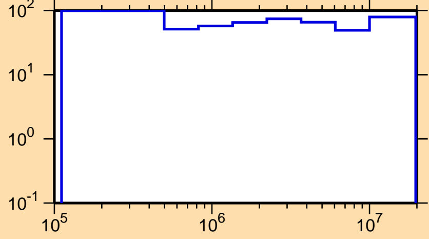
\Delta\sigma/\sigma vs. E for ^{227}\text{Rn}(n,\text{inel.})
