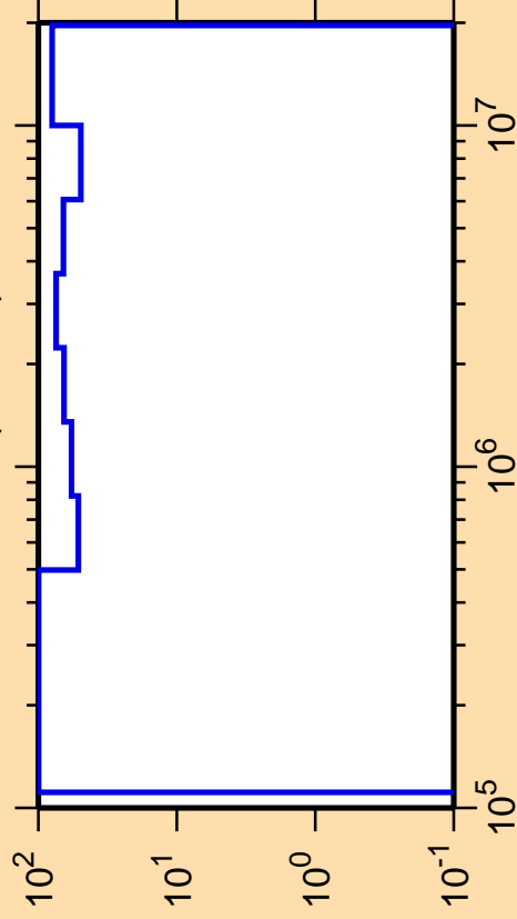
\Delta\sigma/\sigma vs. E for ^{227}\text{Rn}(n,\text{inel.})
