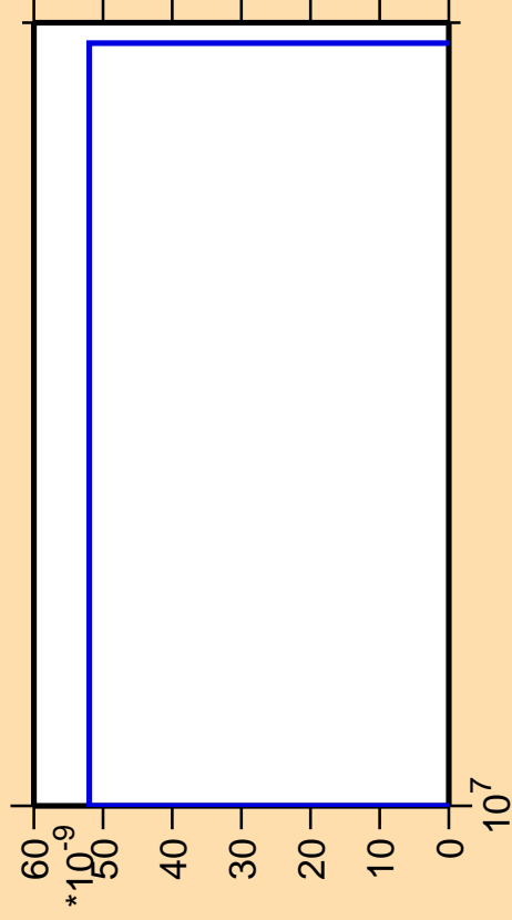
\Delta\sigma/\sigma vs. E for ^{227}\text{Rn} (mt 42)
