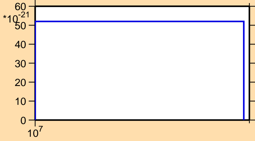
\sigma vs. E for ^{227}\text{Rn} (mt 42)
