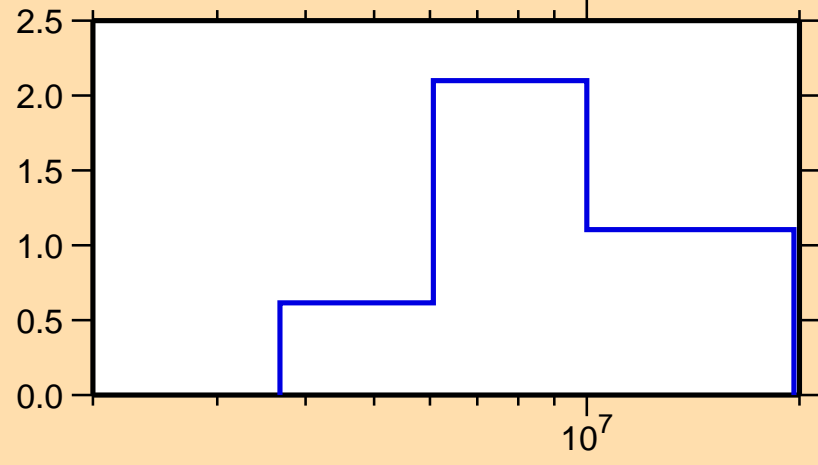
\sigma vs. E for ^{227}\text{Rn}(n,2n)
