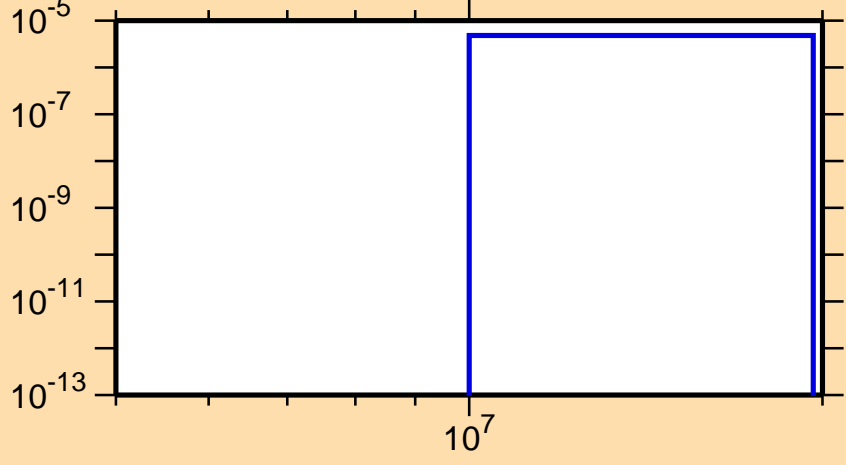
\sigma vs. E for ^{227}\text{Rn}(n,d)
