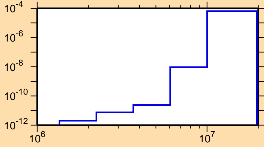
\sigma vs. E for ^{227}\text{Rn}(n,\alpha)
