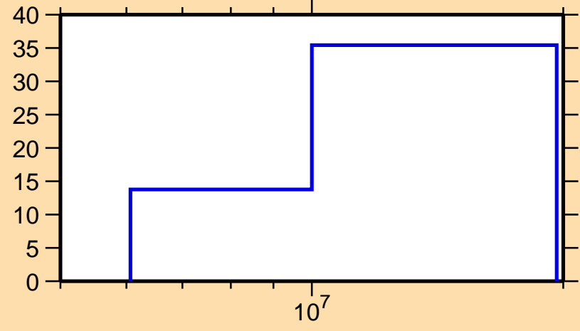
\Delta\sigma/\sigma vs. E for ^{227}\text{Rn}(n,el.)
