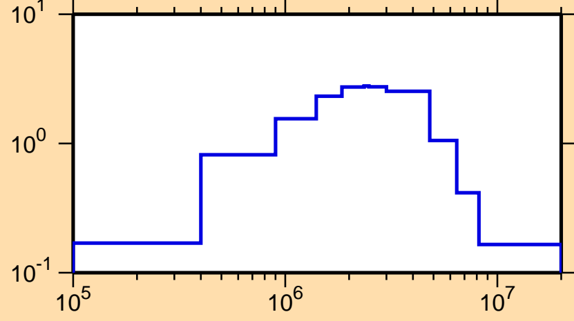
\sigma vs. E for ^{227}\text{Rn}(n,\text{inel.})
