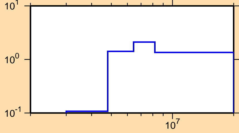
\sigma vs. E for ^{227}\text{Rn}(n,2n)
