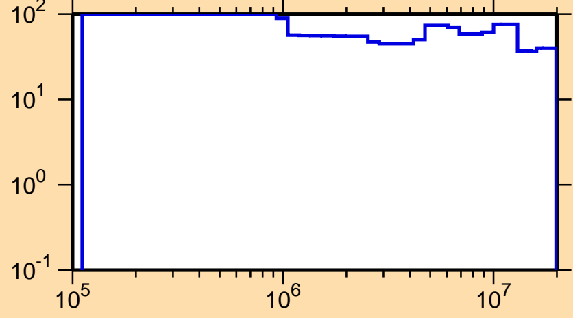
\Delta\sigma/\sigma vs. E for ^{228}\text{Rn}(n,\text{inel.})
