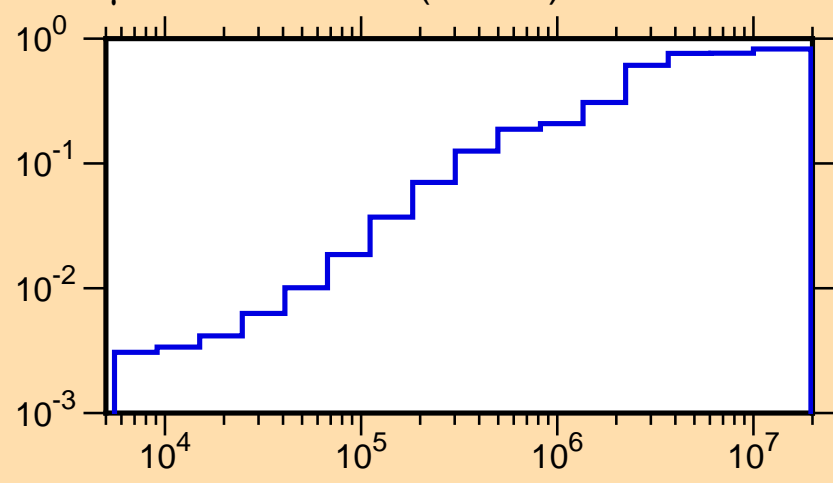
\mu vs. E for ^{228}\text{Rn}(\text{mt251})
