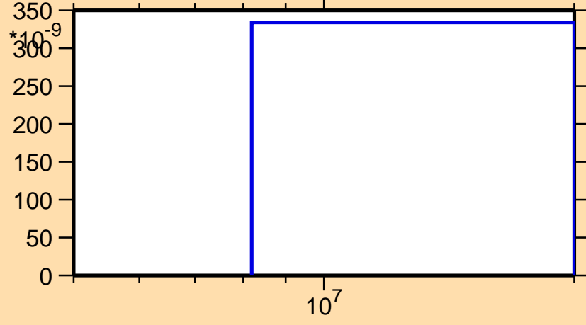
\sigma vs. E for ^{228}\text{Rn}(n,np)
