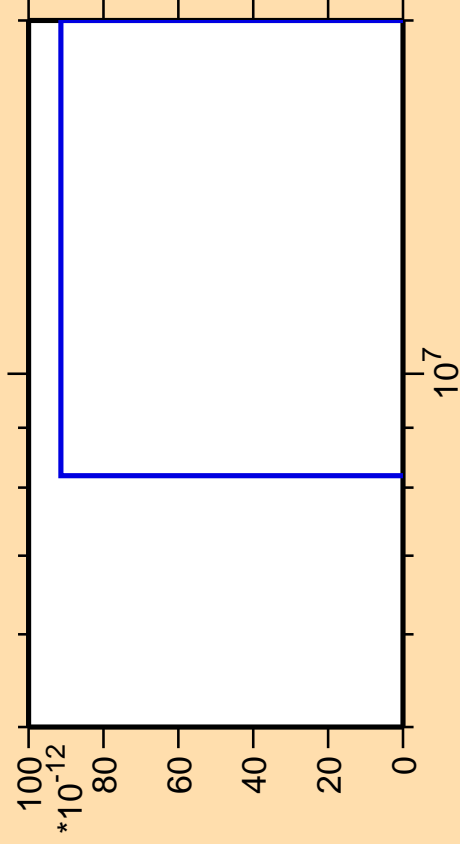
\Delta\sigma/\sigma vs. E for ^{228}\text{Rn}(\text{mt } 42)
