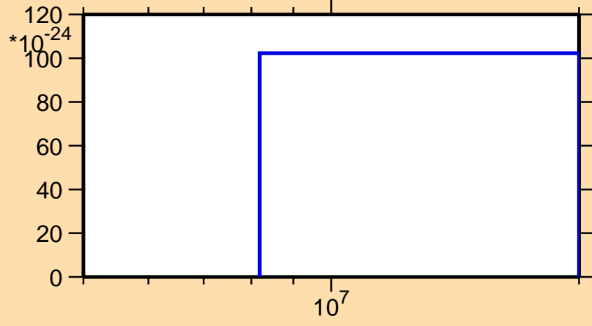
\sigma vs. E for ^{228}\text{Rn}(\text{mt } 42)
