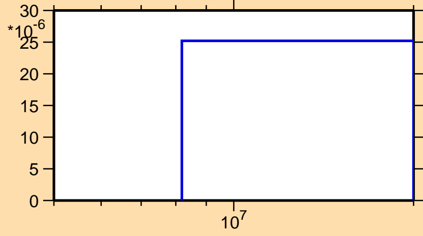
\sigma vs. E for ^{228}\text{Rn}(n,p)
