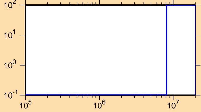
\Delta\sigma/\sigma vs. E for ^{228}\text{Rn}(n,f)
