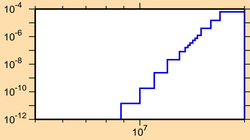
\sigma vs. E for ^{229}\text{Rn}(n,n\alpha)
