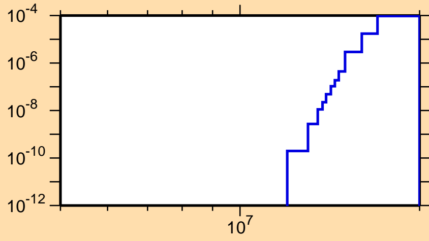
\sigma vs. E for ^{229}\text{Rn}(n,d)
