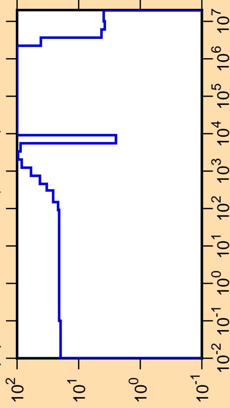
\Delta\mu/\mu vs. E for ^{229}\text{Rn}(\text{mt251})
