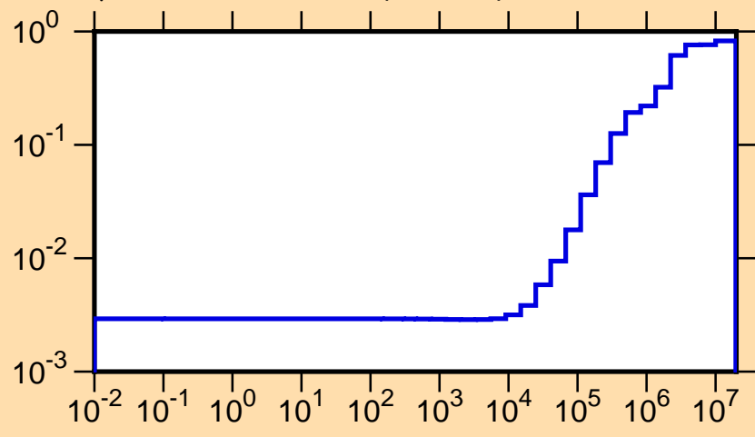
\mu vs. E for ^{229}\text{Rn}(\text{mt251})
