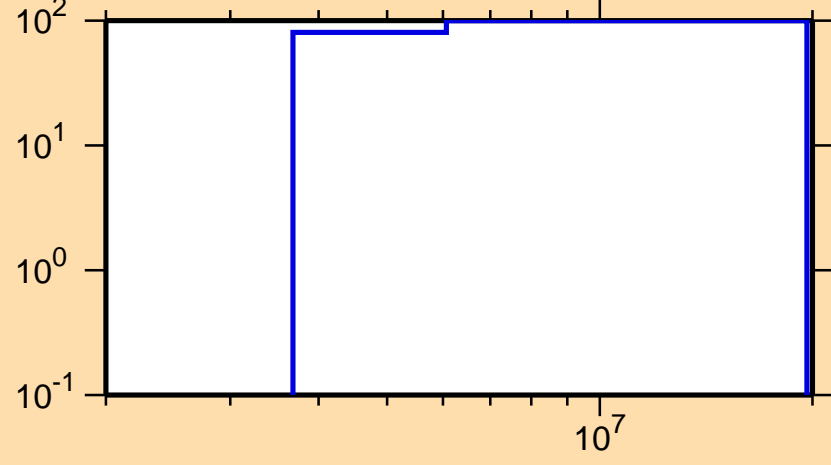
\Delta\sigma/\sigma vs. E for ^{229}\text{Rn}(n,\text{inel.})
