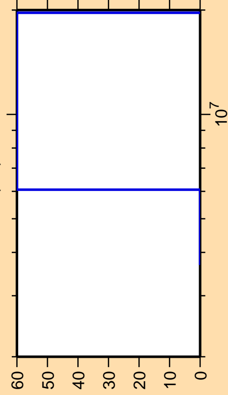
\Delta\sigma/\sigma vs. E for ^{229}\text{Rn}(n,f)
