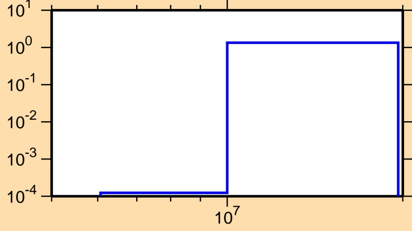
\sigma vs. E for ^{229}\text{Rn}(n,3n)
