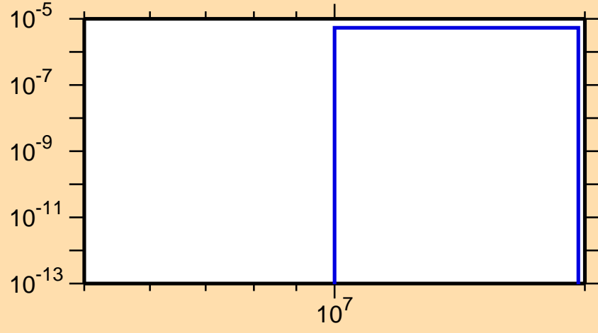
\sigma vs. E for ^{229}\text{Rn}(n,t)
