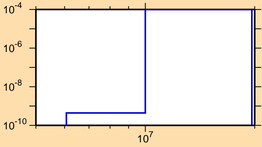
\sigma vs. E for ^{229}\text{Rn}(n,p)
