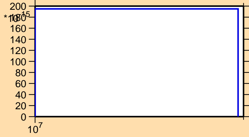
\sigma vs. E for ^{229}\text{Rn}(n,3n\alpha)
