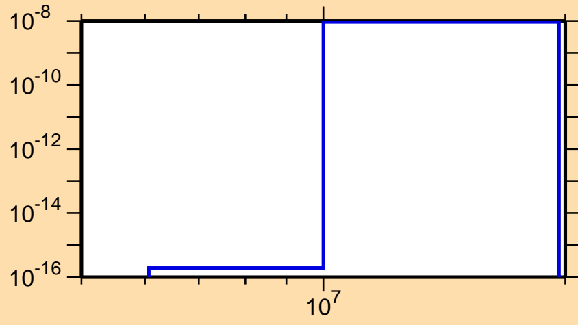
\sigma vs. E for ^{229}\text{Rn}(n,2n\alpha)
