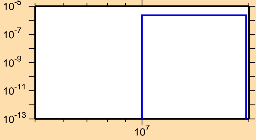
\sigma vs. E for ^{229}\text{Rn}(n,d)
