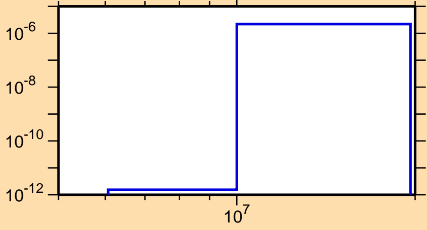
\sigma vs. E for ^{229}\text{Rn}(n,n\alpha)
