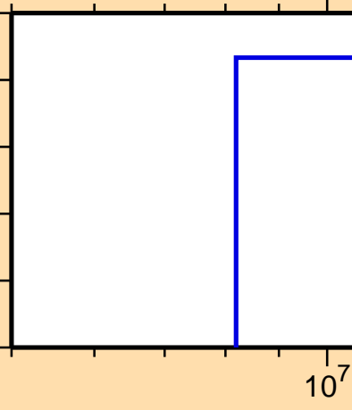
\sigma vs. E for ^{229}\text{Rn}(n,t)
