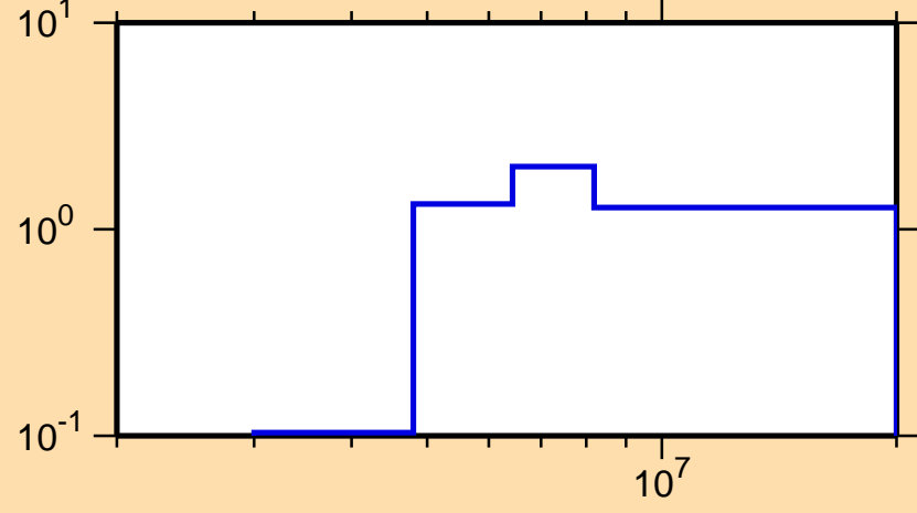
\sigma vs. E for ^{229}\text{Rn}(n,2n)
