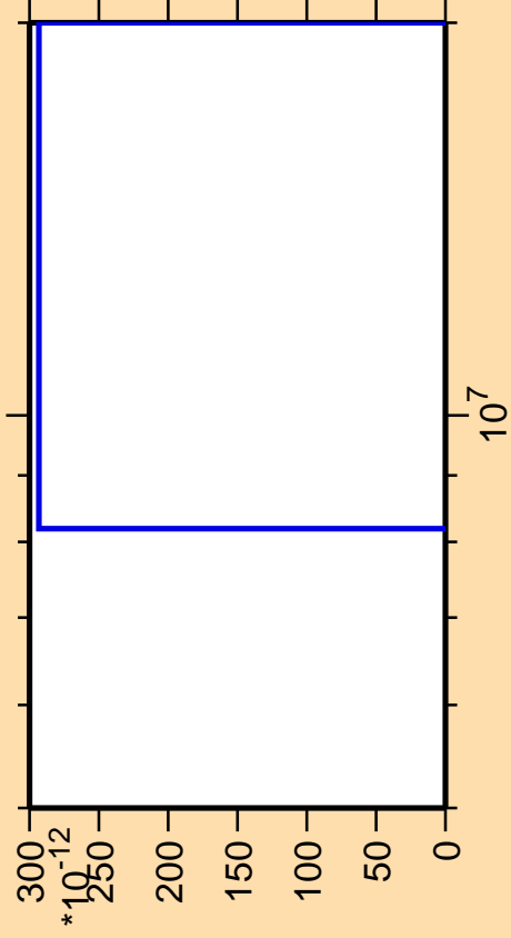
\Delta\sigma/\sigma vs. E for ^{229}\text{Rn}(\text{mt } 42)
