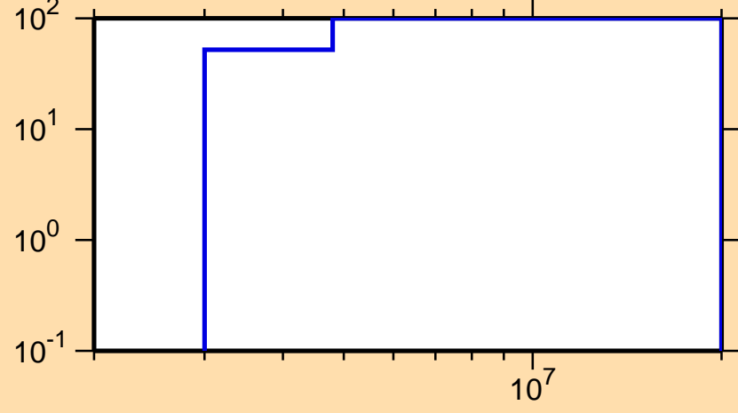
\Delta\sigma/\sigma vs. E for ^{229}\text{Rn}(n,n\text{cont.})
