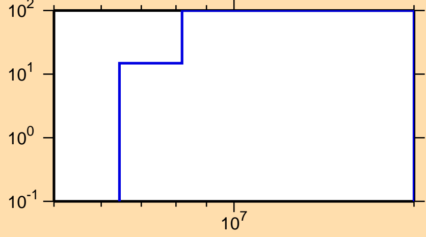
\Delta\sigma/\sigma vs. E for ^{229}\text{Rn}(n,f)
