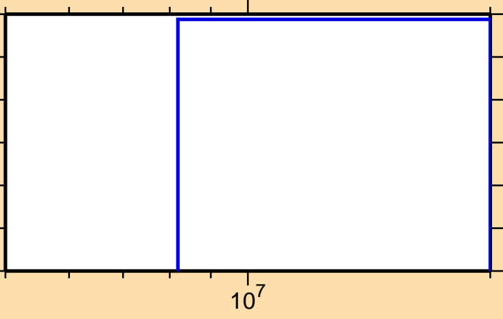
\sigma vs. E for ^{229}\text{Rn}(\text{mt } 42)
