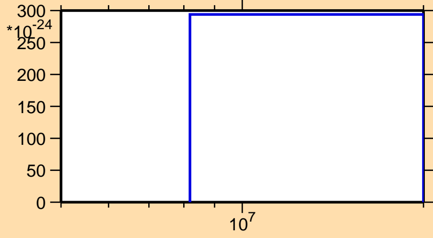
\sigma vs. E for ^{229}\text{Rn}(\text{mt } 42)
