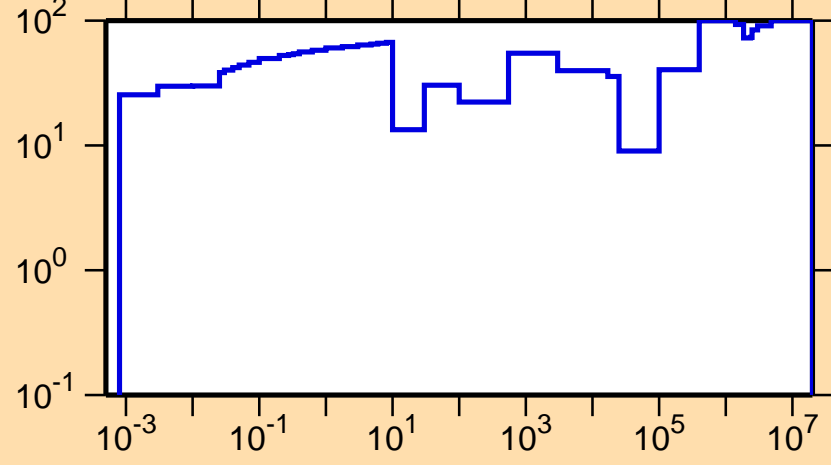
\Delta\sigma/\sigma vs. E for ^{229}\text{Rn}(n,\text{tot.})
