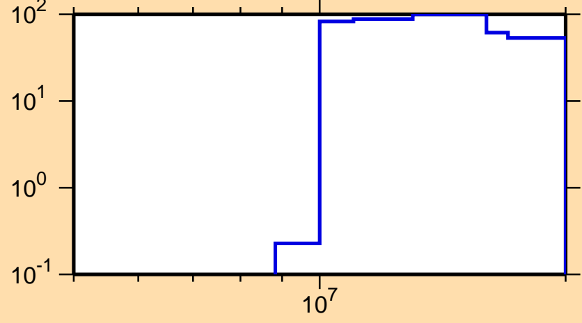
\Delta\sigma/\sigma vs. E for ^{230}\text{Rn}(n,f)
