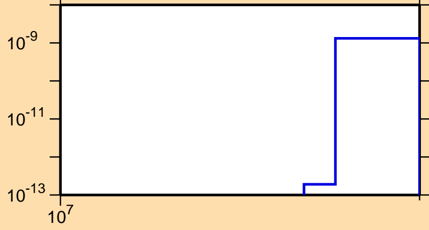
\sigma vs. E for ^{230}\text{Rn}(n,\text{nd})
