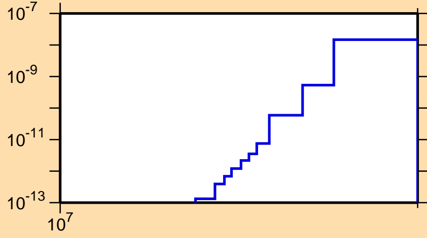
\sigma vs. E for ^{230}\text{Rn}(n,2n\alpha)
