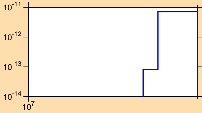
\sigma vs. E for ^{230}\text{Rn}(n,3n\alpha)
