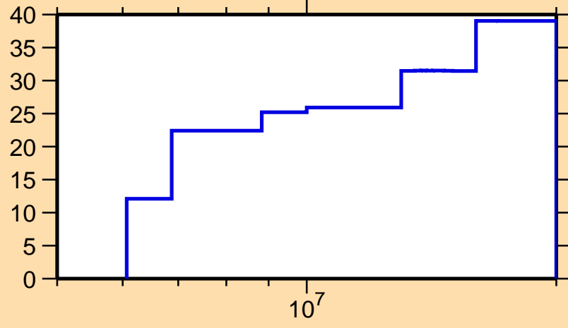
\Delta\sigma/\sigma vs. E for ^{230}\text{Rn}(n,\text{nonel.})
