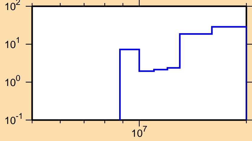
\Delta\sigma/\sigma vs. E for ^{230}\text{Rn}(n,n_1)
